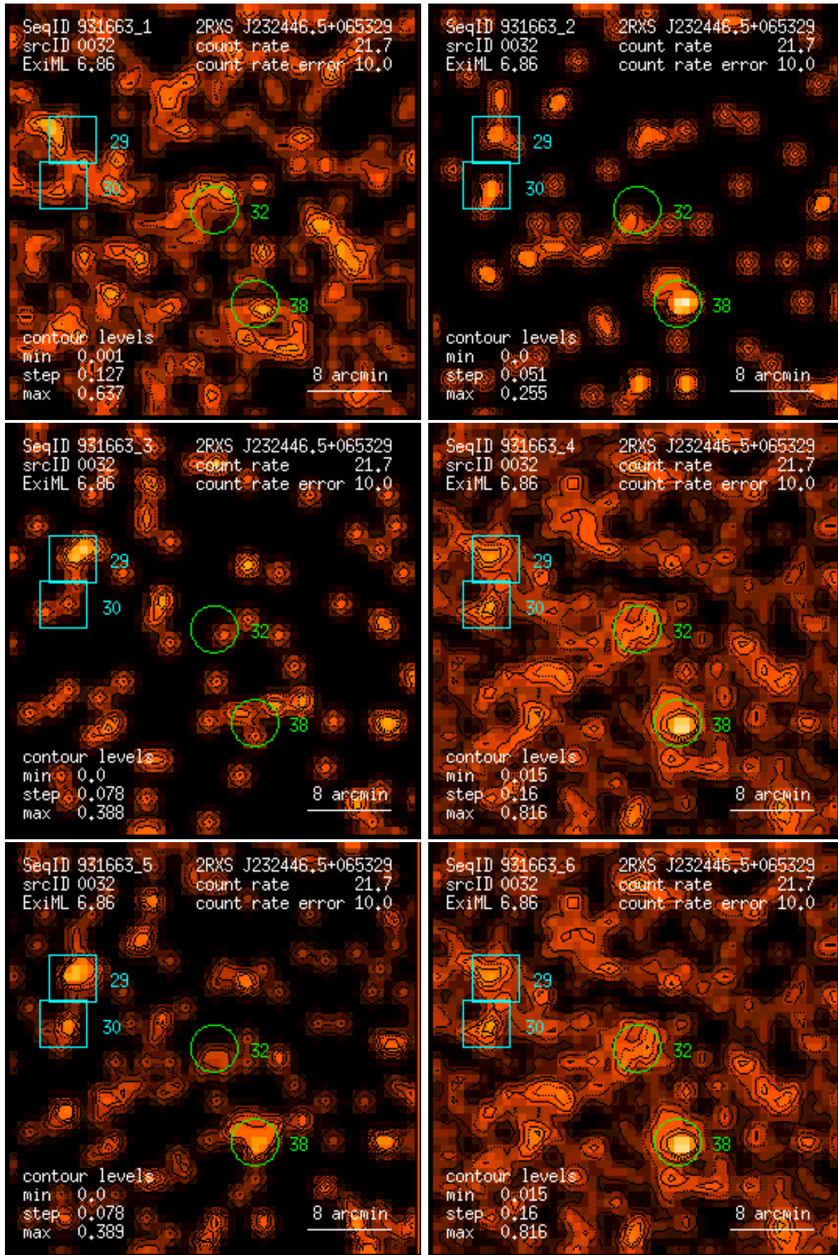
Figure 32: RASS 931663: detection 0032: band rate images, Gaussian filter: (1) PSPC channels 11 – 41, (2) 52 – 90, (3) 91 – 201, (4) 11 – 235, (5) 52 – 201, (6) 11 – 201. Broad band rates in counts/ks. Band rate contour levels in counts/ks/arcmin 2 .
