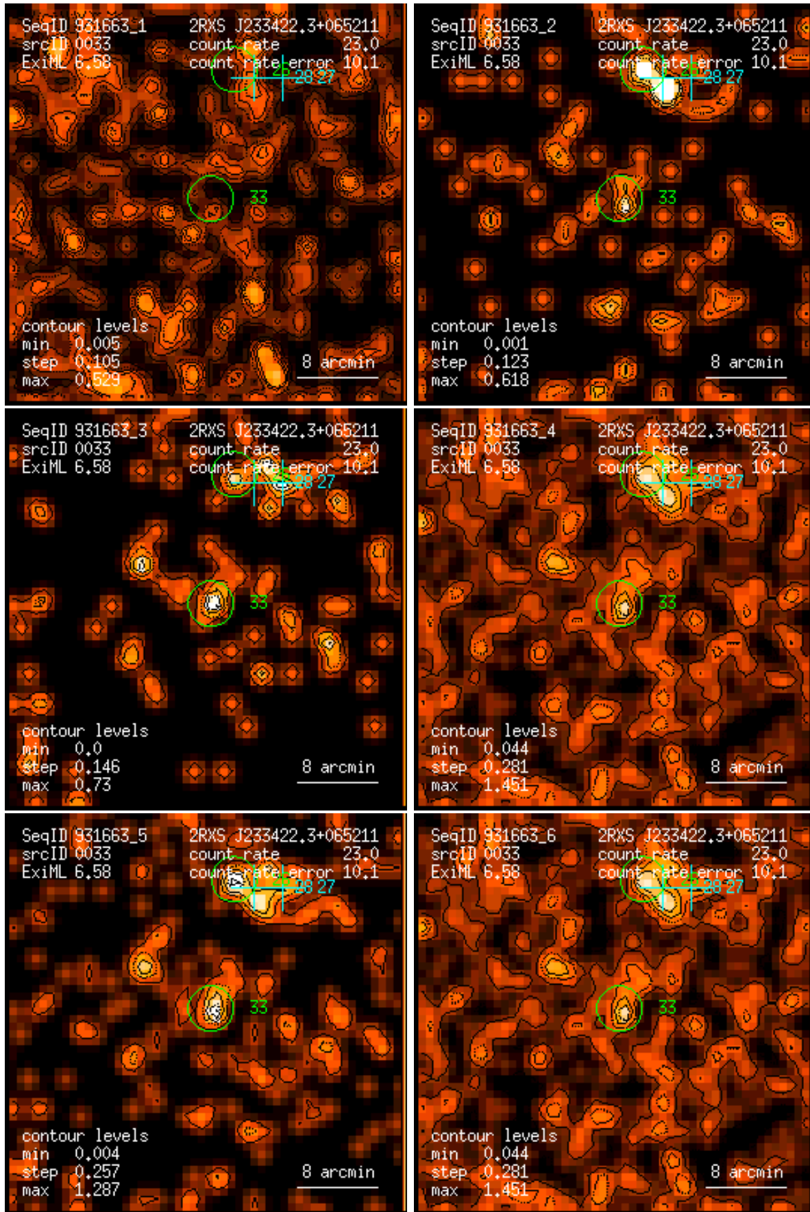
Figure 33: RASS 931663: detection 0033: band rate images, Gaussian filter: (1) PSPC channels 11 – 41, (2) 52 – 90, (3) 91 – 201, (4) 11 – 235, (5) 52 – 201, (6) 11 – 201. Broad band rates in counts/ks. Band rate contour levels in counts/ks/arcmin 2 .
