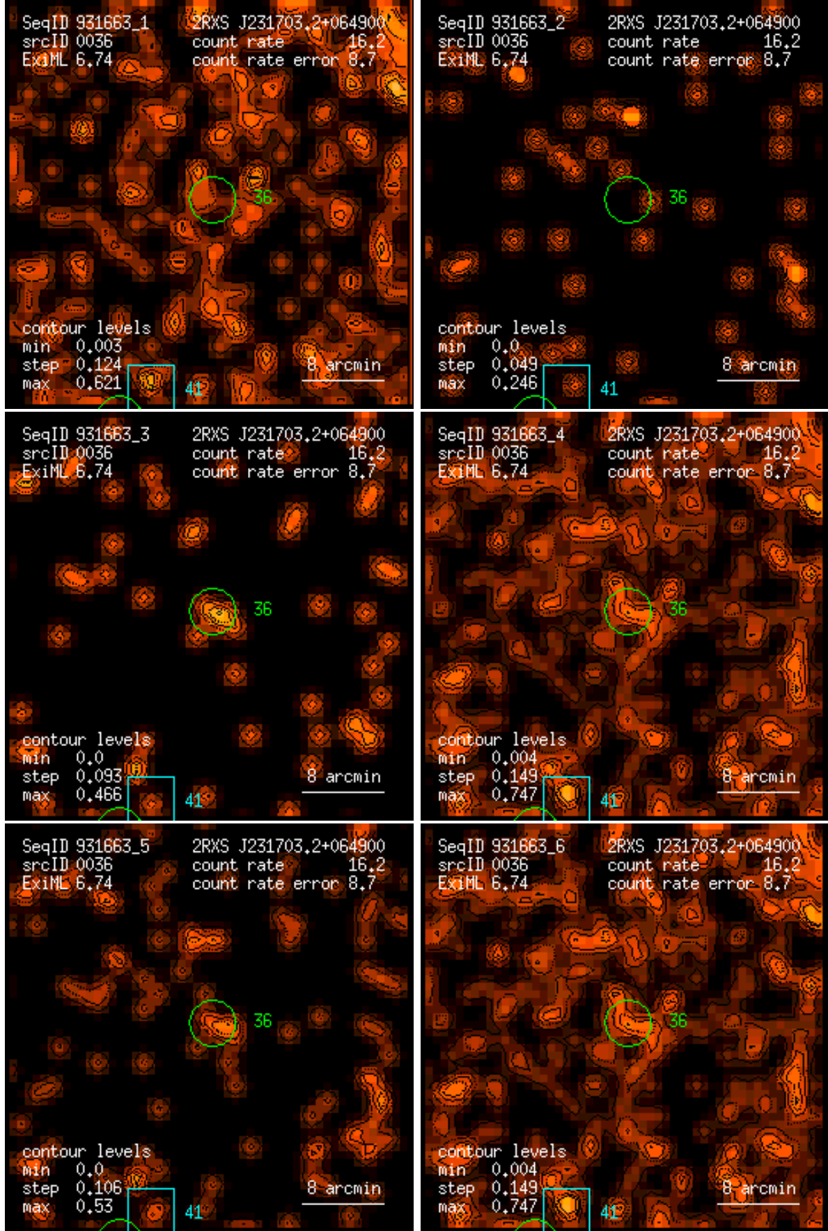
Figure 36: RASS 931663: detection 0036: band rate images, Gaussian filter: (1) PSPC channels 11 – 41, (2) 52 – 90, (3) 91 – 201, (4) 11 – 235, (5) 52 – 201, (6) 11 – 201. Broad band rates in counts/ks. Band rate contour levels in counts/ks/arcmin 2 .
