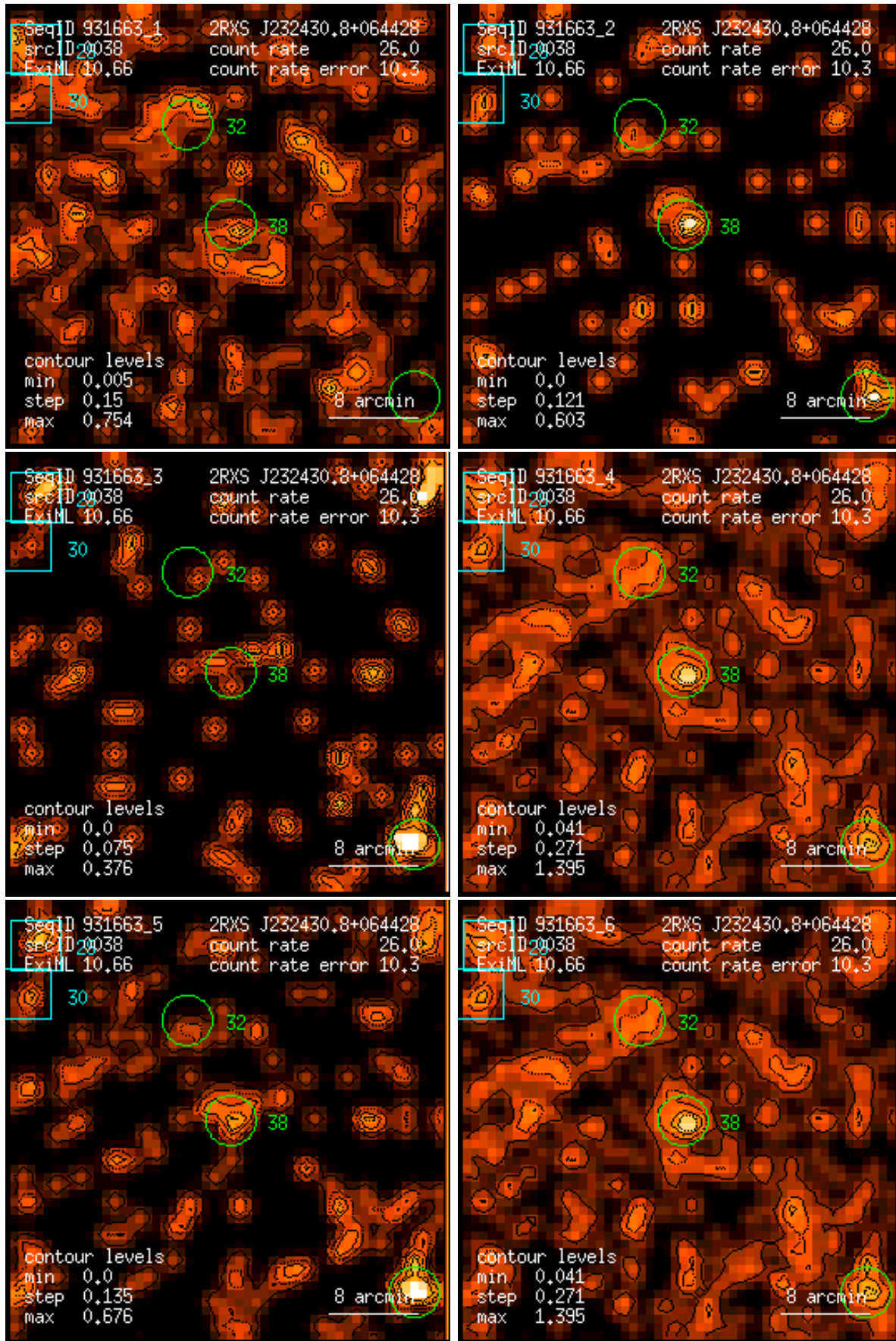
Figure 38: RASS 931663: detection 0038: band rate images, Gaussian filter: (1) PSPC channels 11 – 41, (2) 52 – 90, (3) 91 – 201, (4) 11 – 235, (5) 52 – 201, (6) 11 – 201. Broad band rates in counts/ks. Band rate contour levels in counts/ks/arcmin 2 .
