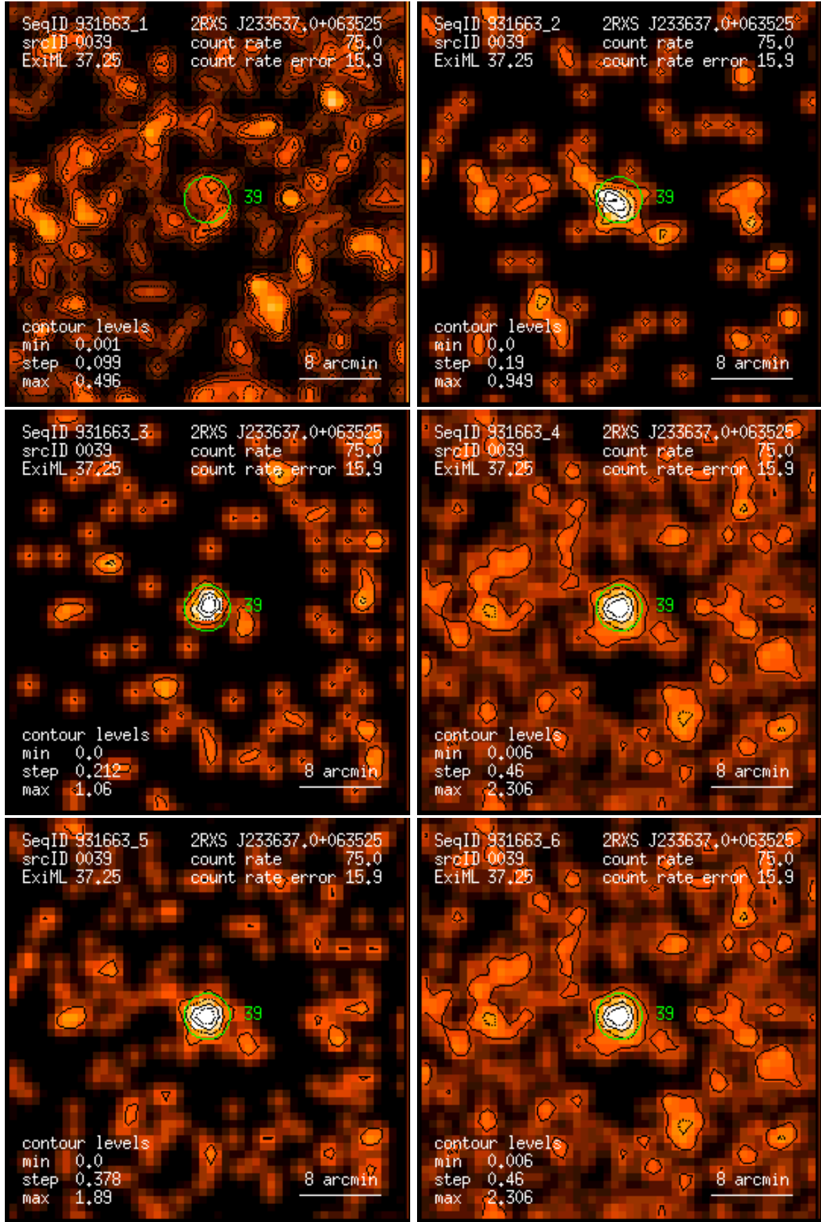
Figure 39: RASS 931663: detection 0039: band rate images, Gaussian filter: (1) PSPC channels 11 – 41, (2) 52 – 90, (3) 91 – 201, (4) 11 – 235, (5) 52 – 201, (6) 11 – 201. Broad band rates in counts/ks. Band rate contour levels in counts/ks/arcmin 2 .
