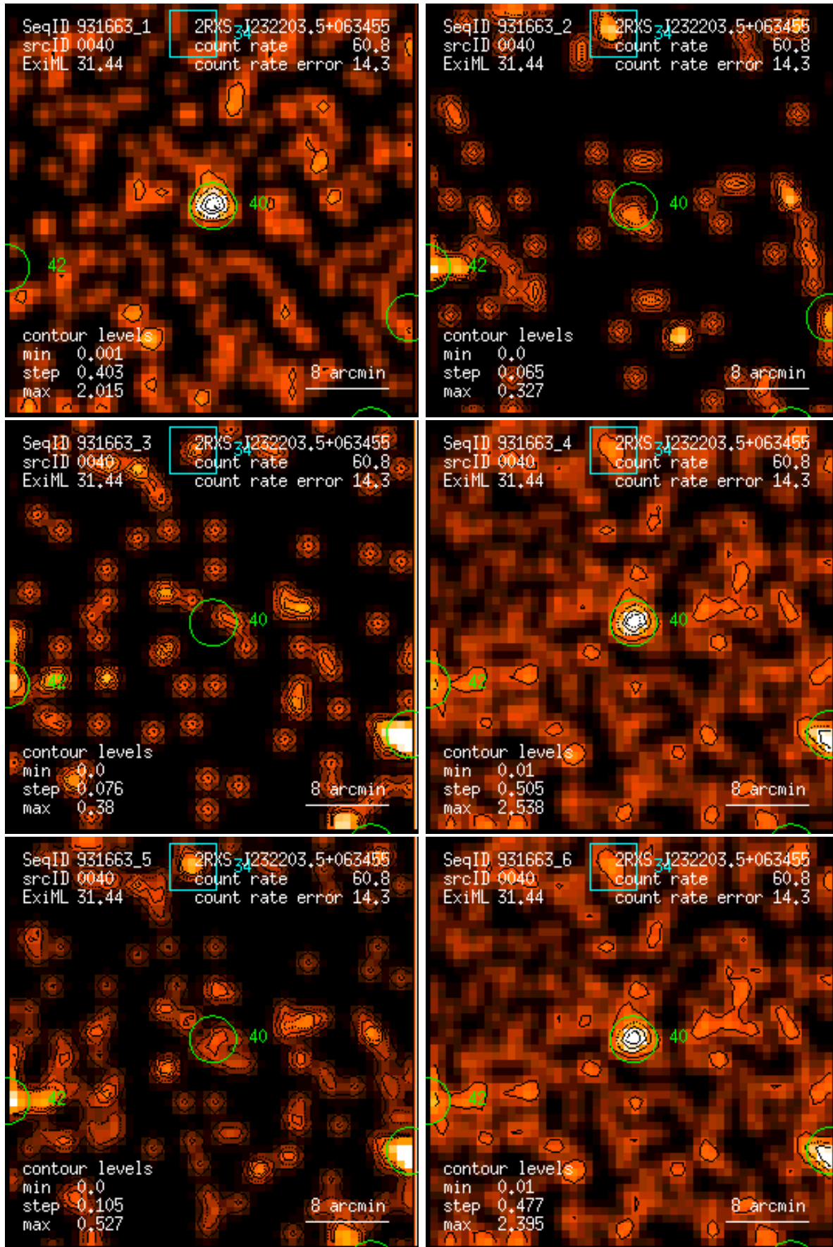
Figure 40: RASS 931663: detection 0040: band rate images, Gaussian filter: (1) PSPC channels 11 – 41, (2) 52 – 90, (3) 91 – 201, (4) 11 – 235, (5) 52 – 201, (6) 11 – 201. Broad band rates in counts/ks. Band rate contour levels in counts/ks/arcmin 2 .
