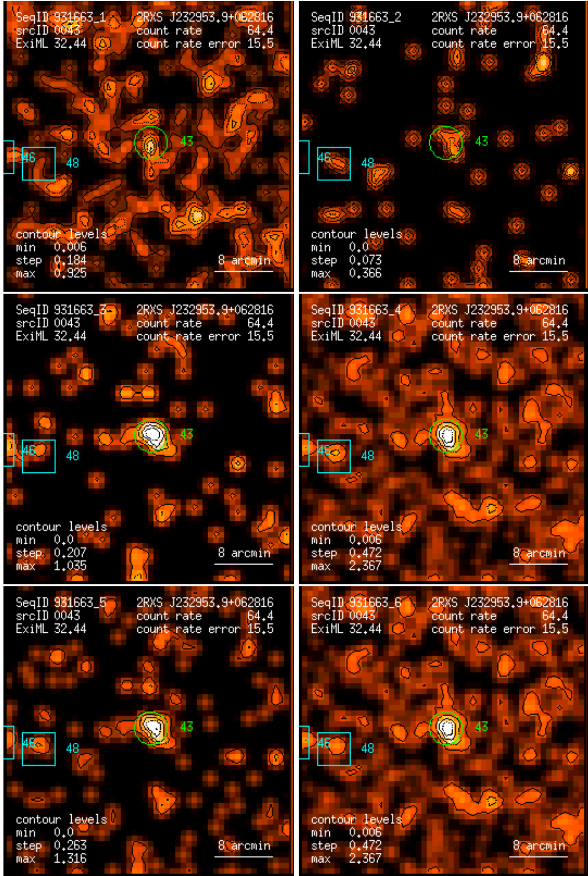
Figure 43: RASS 931663: detection 0043: band rate images, Gaussian filter: (1) PSPC channels 11 – 41, (2) 52 – 90, (3) 91 – 201, (4) 11 – 235, (5) 52 – 201, (6) 11 – 201. Broad band rates in counts/ks. Band rate contour levels in counts/ks/arcmin 2 .
