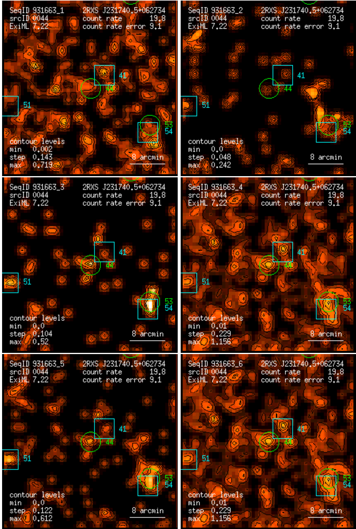
Figure 44: RASS 931663: detection 0044: band rate images, Gaussian filter: (1) PSPC channels 11 – 41, (2) 52 – 90, (3) 91 – 201, (4) 11 – 235, (5) 52 – 201, (6) 11 – 201. Broad band rates in counts/ks. Band rate contour levels in counts/ks/arcmin 2 .
