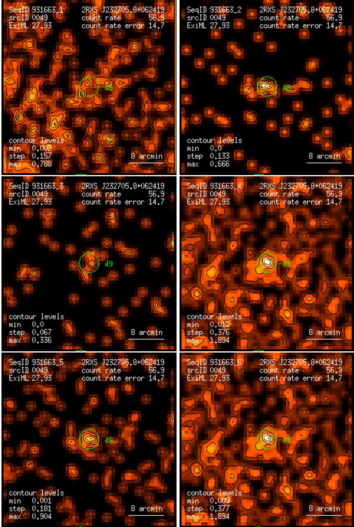
Figure 49: RASS 931663: detection 0049: band rate images, Gaussian filter: (1) PSPC channels 11 – 41, (2) 52 – 90, (3) 91 – 201, (4) 11 – 235, (5) 52 – 201, (6) 11 – 201. Broad band rates in counts/ks. Band rate contour levels in counts/ks/arcmin 2 .
