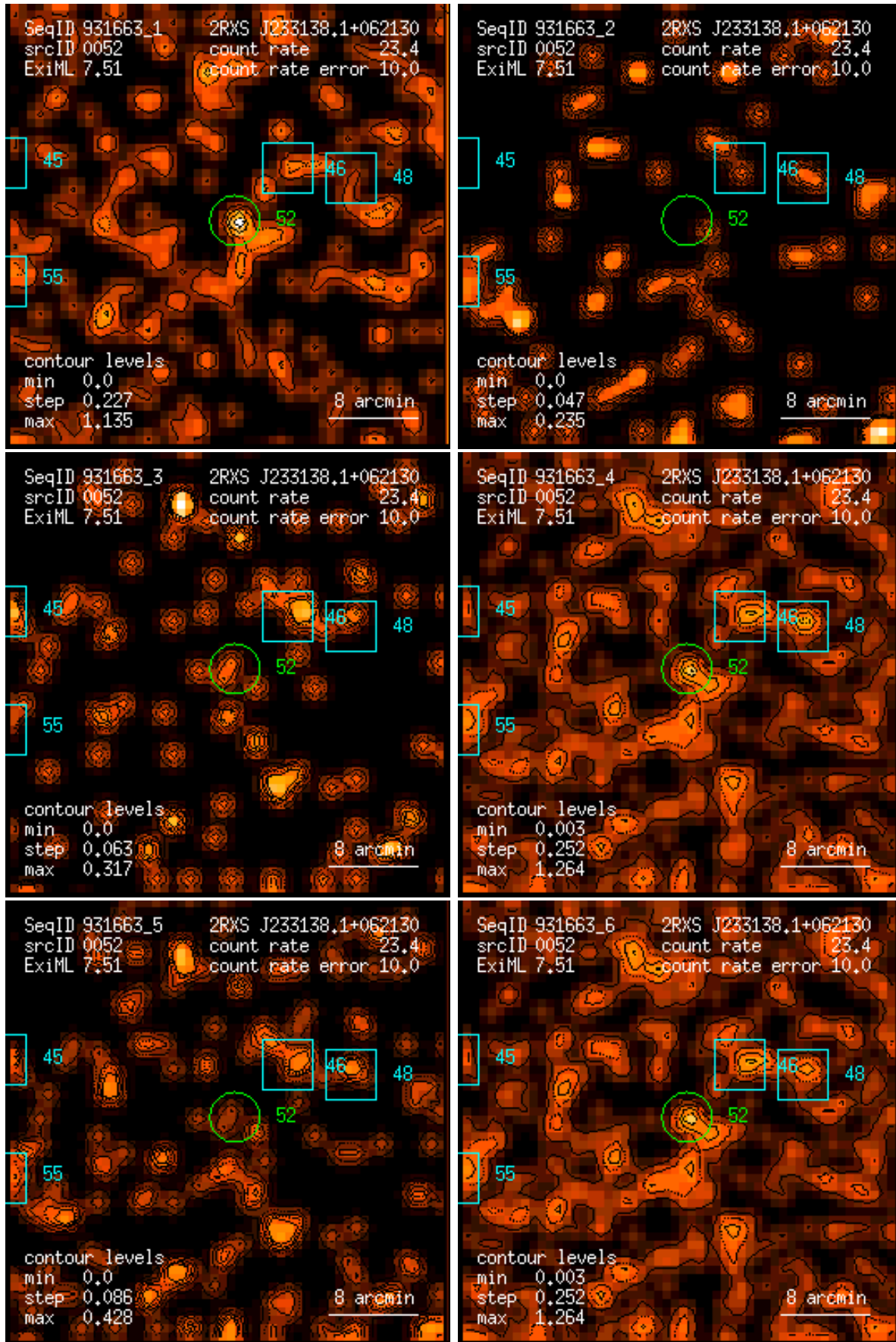
Figure 52: RASS 931663: detection 0052: band rate images, Gaussian filter: (1) PSPC channels 11 – 41, (2) 52 – 90, (3) 91 – 201, (4) 11 – 235, (5) 52 – 201, (6) 11 – 201. Broad band rates in counts/ks. Band rate contour levels in counts/ks/arcmin 2 .
