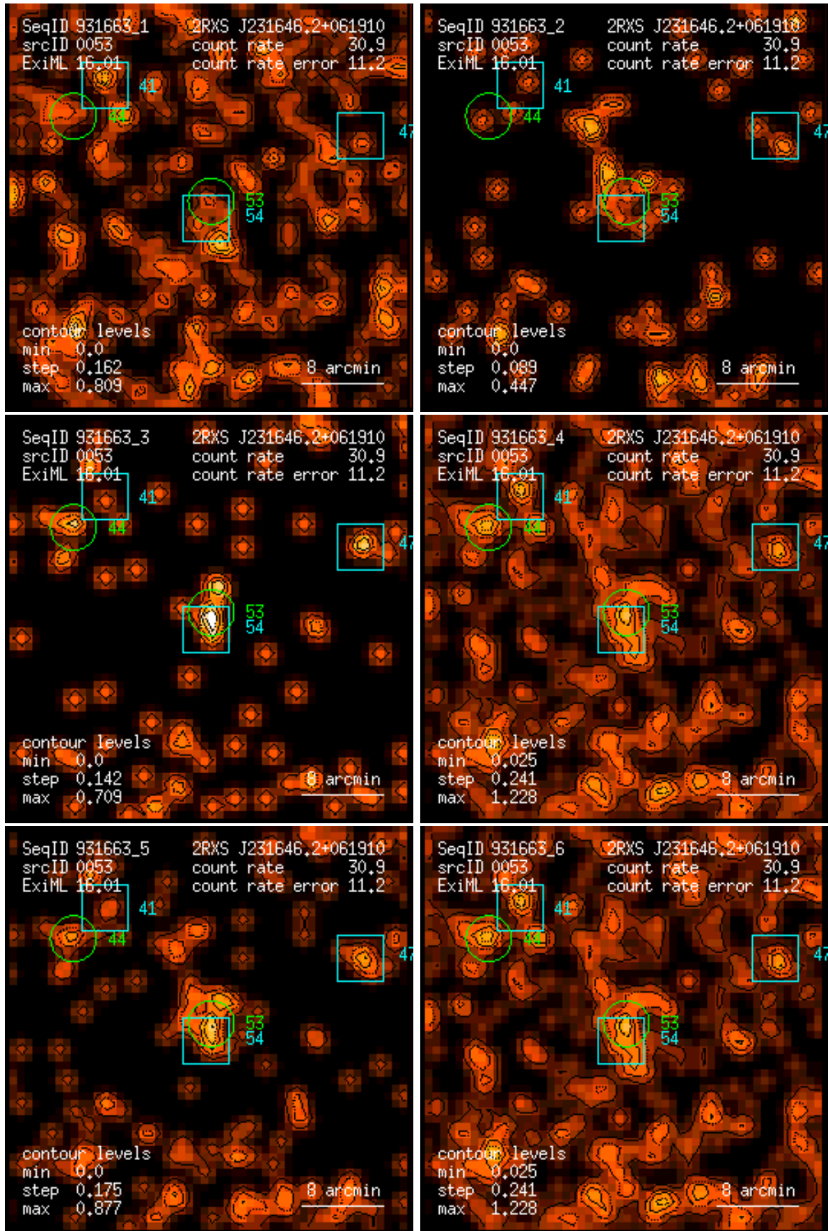
Figure 53: RASS 931663: detection 0053: band rate images, Gaussian filter: (1) PSPC channels 11 – 41, (2) 52 – 90, (3) 91 – 201, (4) 11 – 235, (5) 52 – 201, (6) 11 – 201. Broad band rates in counts/ks. Band rate contour levels in counts/ks/arcmin 2 .
