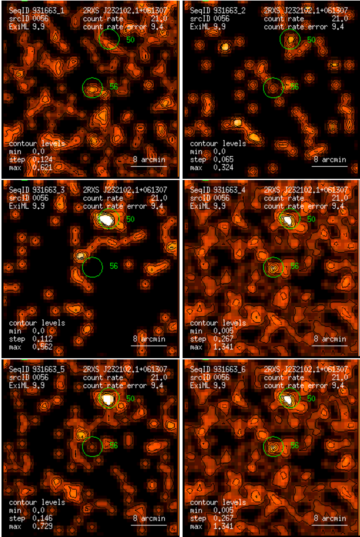
Figure 56: RASS 931663: detection 0056: band rate images, Gaussian filter: (1) PSPC channels 11 – 41, (2) 52 – 90, (3) 91 – 201, (4) 11 – 235, (5) 52 – 201, (6) 11 – 201. Broad band rates in counts/ks. Band rate contour levels in counts/ks/arcmin 2 .
