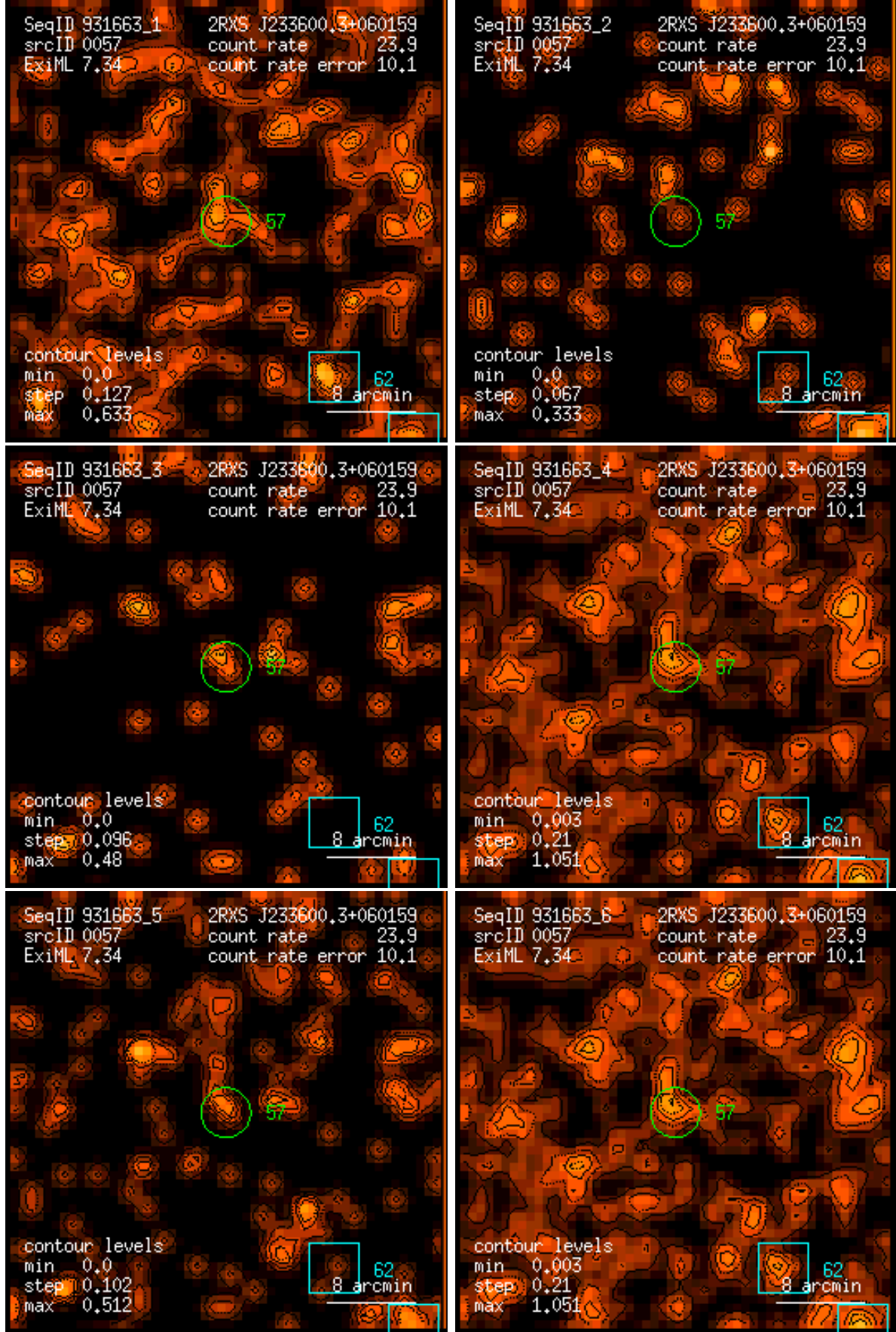
Figure 57: RASS 931663: detection 0057: band rate images, Gaussian filter: (1) PSPC channels 11 – 41, (2) 52 – 90, (3) 91 – 201, (4) 11 – 235, (5) 52 – 201, (6) 11 – 201. Broad band rates in counts/ks. Band rate contour levels in counts/ks/arcmin 2 .
