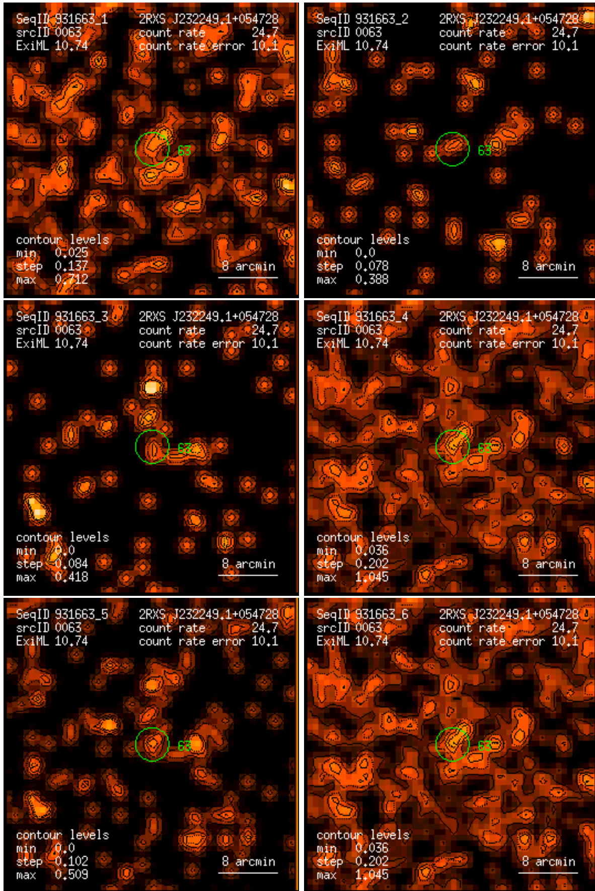
Figure 63: RASS 931663: detection 0063: band rate images, Gaussian filter: (1) PSPC channels 11 – 41, (2) 52 – 90, (3) 91 – 201, (4) 11 – 235, (5) 52 – 201, (6) 11 – 201. Broad band rates in counts/ks. Band rate contour levels in counts/ks/arcmin 2 .
