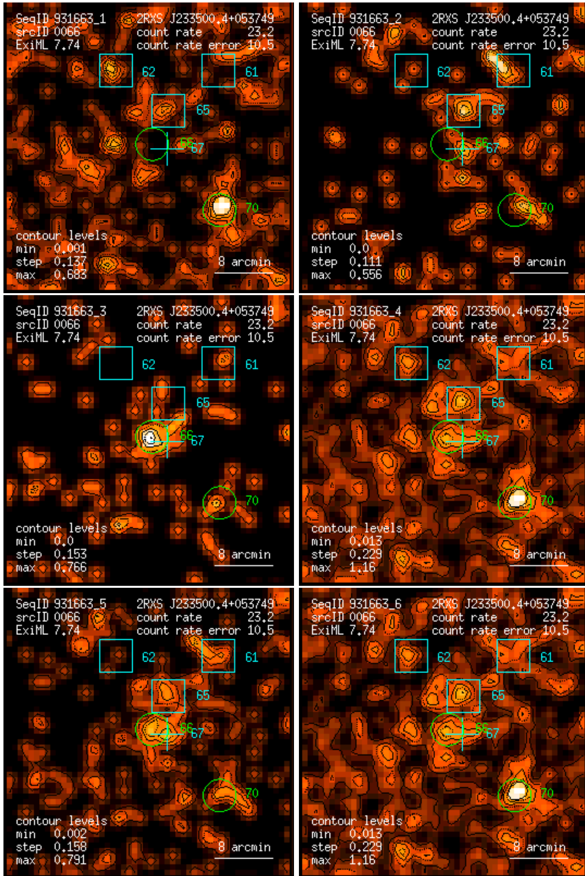
Figure 66: RASS 931663: detection 0066: band rate images, Gaussian filter: (1) PSPC channels 11 – 41, (2) 52 – 90, (3) 91 – 201, (4) 11 – 235, (5) 52 – 201, (6) 11 – 201. Broad band rates in counts/ks. Band rate contour levels in counts/ks/arcmin 2 .
