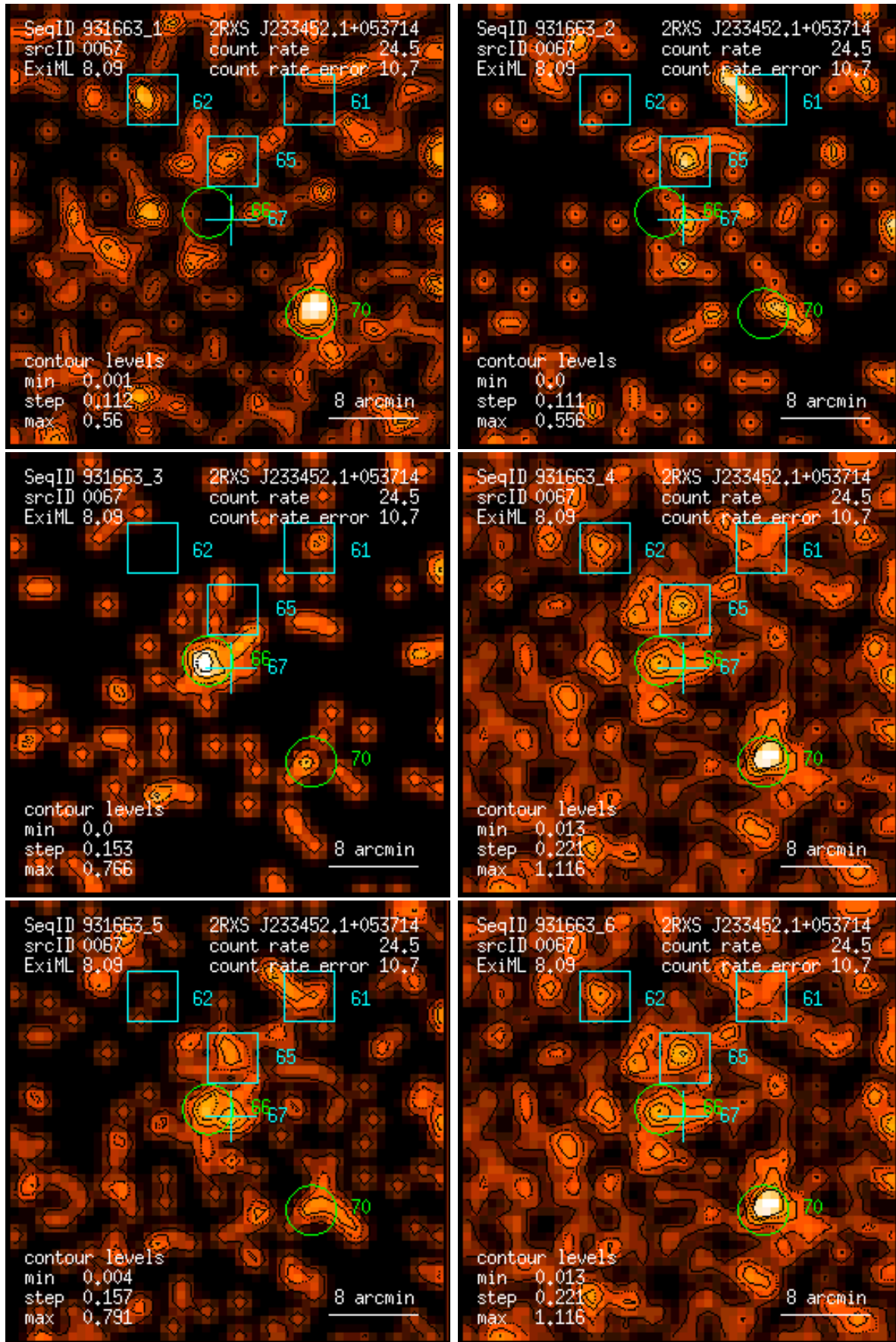
Figure 67: RASS 931663: detection 0067: band rate images, Gaussian filter: (1) PSPC channels 11 – 41, (2) 52 – 90, (3) 91 – 201, (4) 11 – 235, (5) 52 – 201, (6) 11 – 201. Broad band rates in counts/ks. Band rate contour levels in counts/ks/arcmin 2 .
