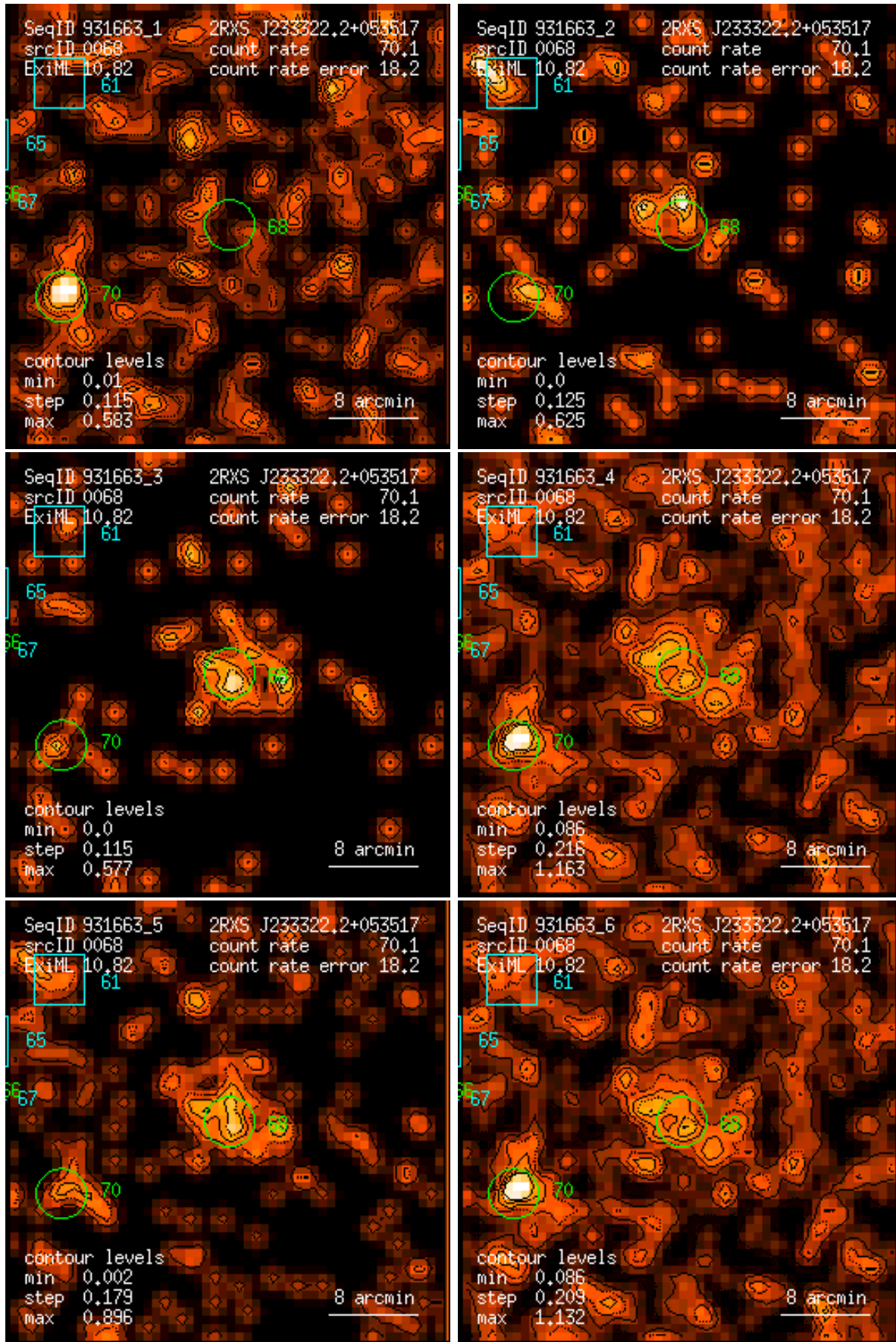
Figure 68: RASS 931663: detection 0068: band rate images, Gaussian filter: (1) PSPC channels 11 – 41, (2) 52 – 90, (3) 91 – 201, (4) 11 – 235, (5) 52 – 201, (6) 11 – 201. Broad band rates in counts/ks. Band rate contour levels in counts/ks/arcmin 2 .
