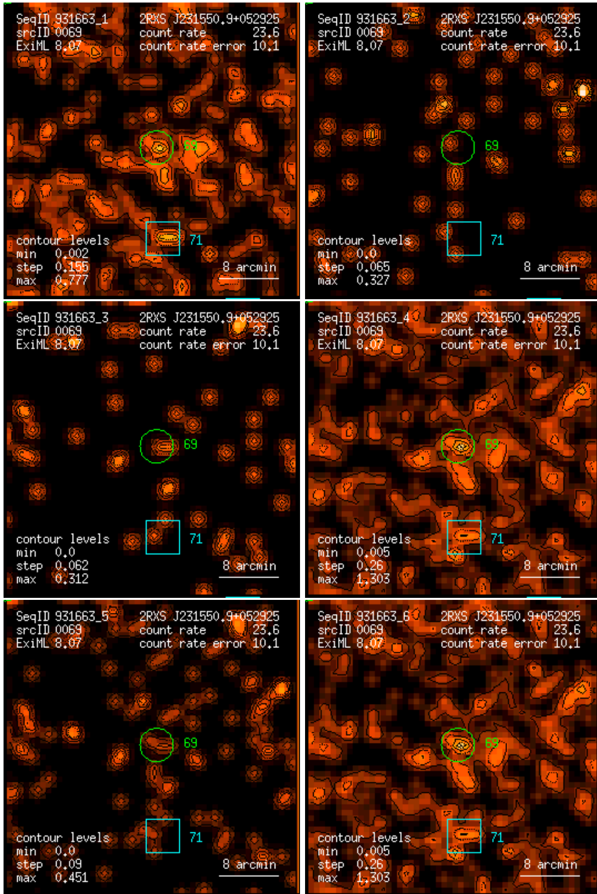
Figure 69: RASS 931663: detection 0069: band rate images, Gaussian filter: (1) PSPC channels 11 – 41, (2) 52 – 90, (3) 91 – 201, (4) 11 – 235, (5) 52 – 201, (6) 11 – 201. Broad band rates in counts/ks. Band rate contour levels in counts/ks/arcmin 2 .
