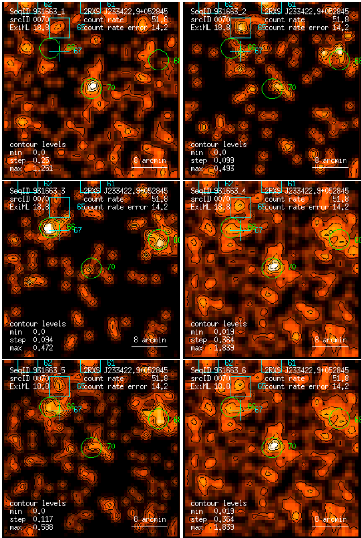
Figure 70: RASS 931663: detection 0070: band rate images, Gaussian filter: (1) PSPC channels 11 – 41, (2) 52 – 90, (3) 91 – 201, (4) 11 – 235, (5) 52 – 201, (6) 11 – 201. Broad band rates in counts/ks. Band rate contour levels in counts/ks/arcmin 2 .
