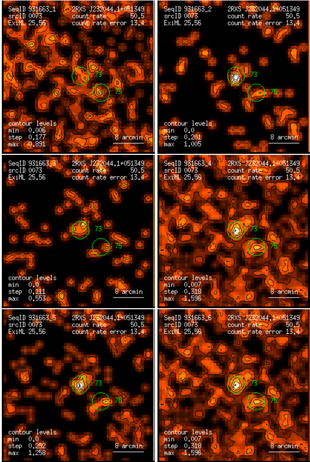
Figure 73: RASS 931663: detection 0073: band rate images, Gaussian filter: (1) PSPC channels 11 – 41, (2) 52 – 90, (3) 91 – 201, (4) 11 – 235, (5) 52 – 201, (6) 11 – 201. Broad band rates in counts/ks. Band rate contour levels in counts/ks/arcmin 2 .
