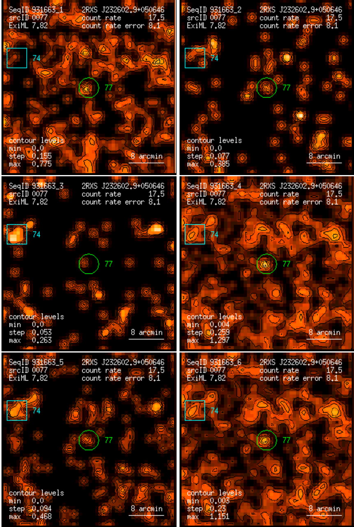
Figure 77: RASS 931663: detection 0077: band rate images, Gaussian filter: (1) PSPC channels 11 – 41, (2) 52 – 90, (3) 91 – 201, (4) 11 – 235, (5) 52 – 201, (6) 11 – 201. Broad band rates in counts/ks. Band rate contour levels in counts/ks/arcmin 2 .
