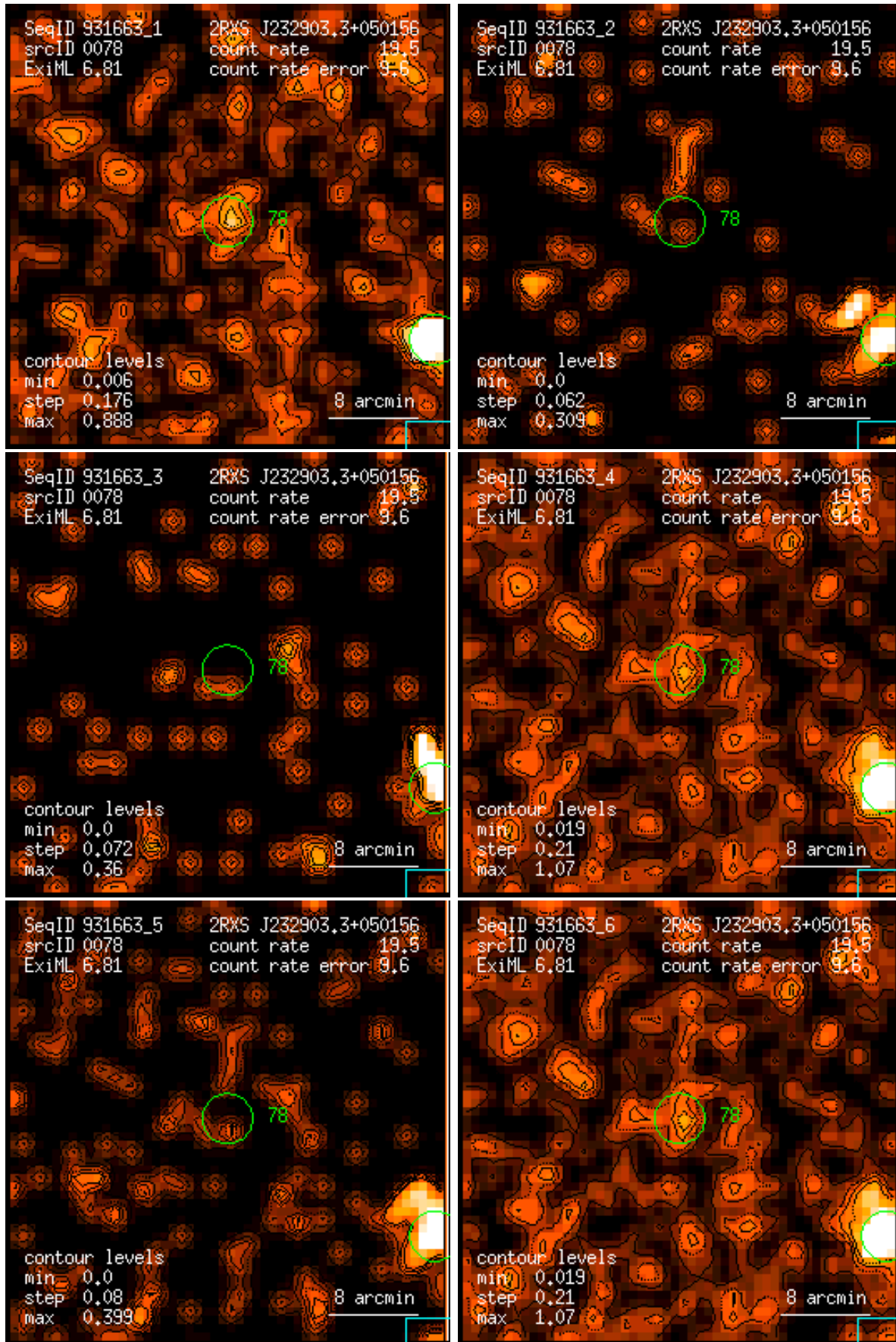
Figure 78: RASS 931663: detection 0078: band rate images, Gaussian filter: (1) PSPC channels 11 – 41, (2) 52 – 90, (3) 91 – 201, (4) 11 – 235, (5) 52 – 201, (6) 11 – 201. Broad band rates in counts/ks. Band rate contour levels in counts/ks/arcmin 2 .
