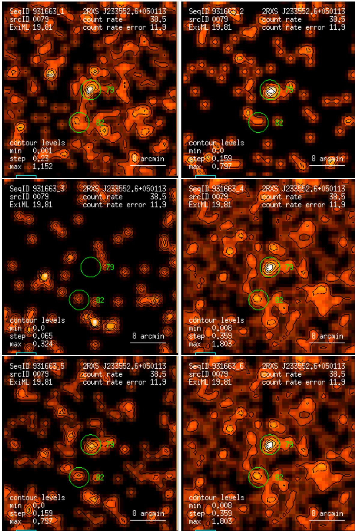
Figure 79: RASS 931663: detection 0079: band rate images, Gaussian filter: (1) PSPC channels 11 – 41, (2) 52 – 90, (3) 91 – 201, (4) 11 – 235, (5) 52 – 201, (6) 11 – 201. Broad band rates in counts/ks. Band rate contour levels in counts/ks/arcmin 2 .
