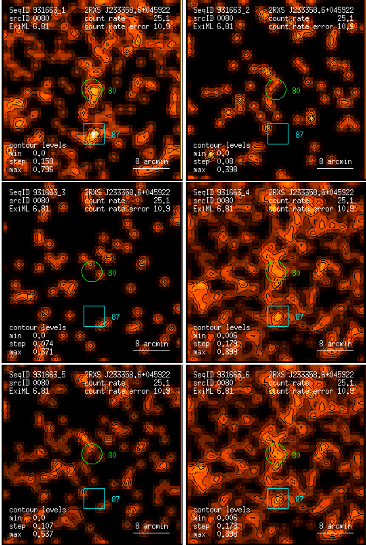
Figure 80: RASS 931663: detection 0080: band rate images, Gaussian filter: (1) PSPC channels 11 – 41, (2) 52 – 90, (3) 91 – 201, (4) 11 – 235, (5) 52 – 201, (6) 11 – 201. Broad band rates in counts/ks. Band rate contour levels in counts/ks/arcmin 2 .
