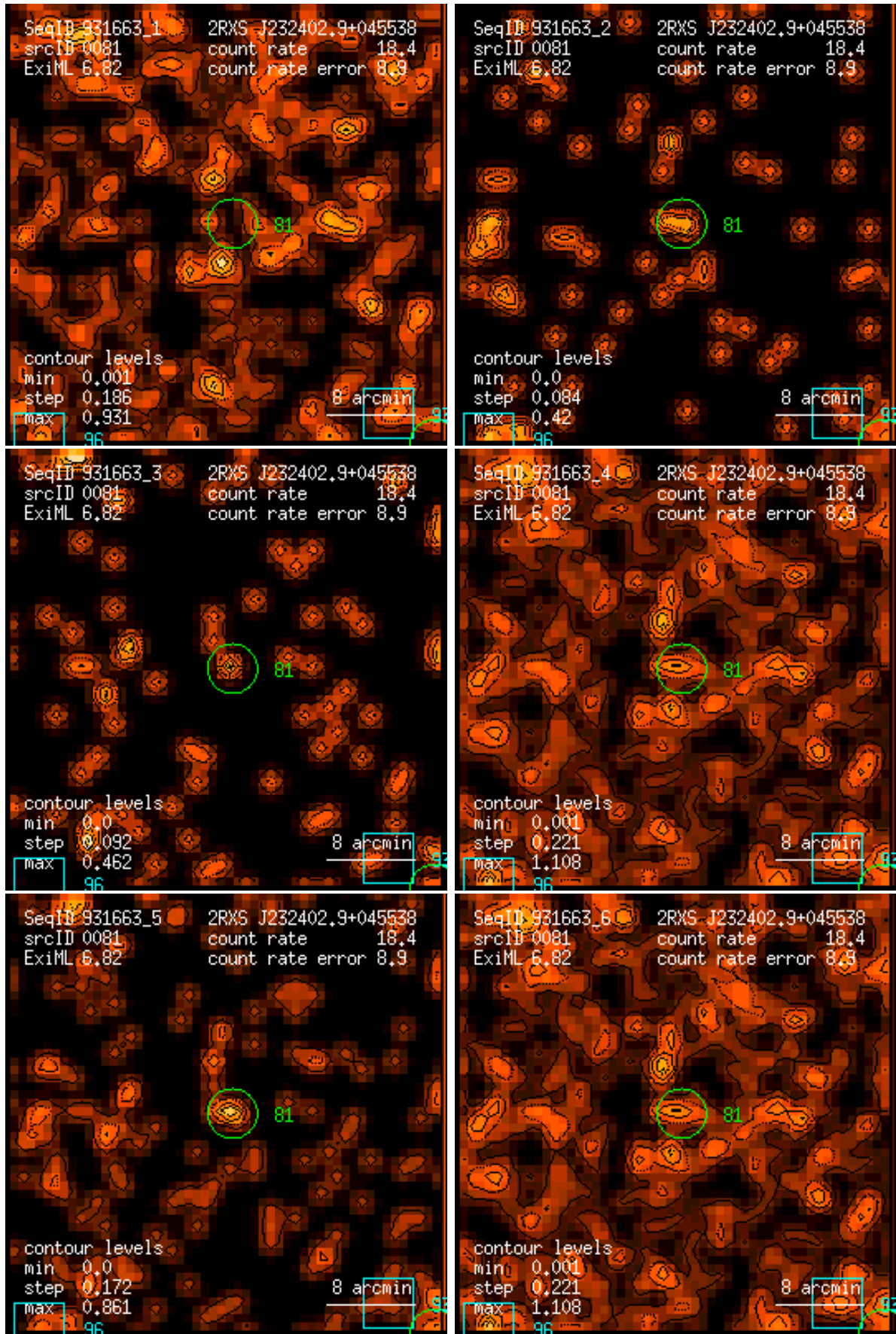
Figure 81: RASS 931663: detection 0081: band rate images, Gaussian filter: (1) PSPC channels 11 – 41, (2) 52 – 90, (3) 91 – 201, (4) 11 – 235, (5) 52 – 201, (6) 11 – 201. Broad band rates in counts/ks. Band rate contour levels in counts/ks/arcmin 2 .
