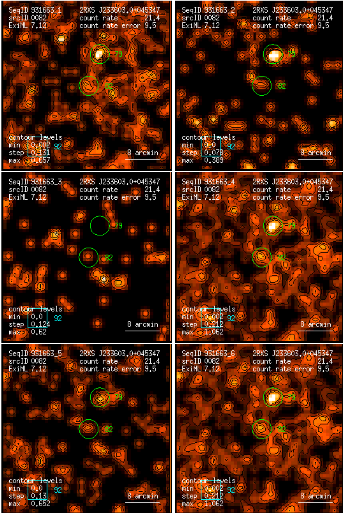
Figure 82: RASS 931663: detection 0082: band rate images, Gaussian filter: (1) PSPC channels 11 – 41, (2) 52 – 90, (3) 91 – 201, (4) 11 – 235, (5) 52 – 201, (6) 11 – 201. Broad band rates in counts/ks. Band rate contour levels in counts/ks/arcmin 2 .
