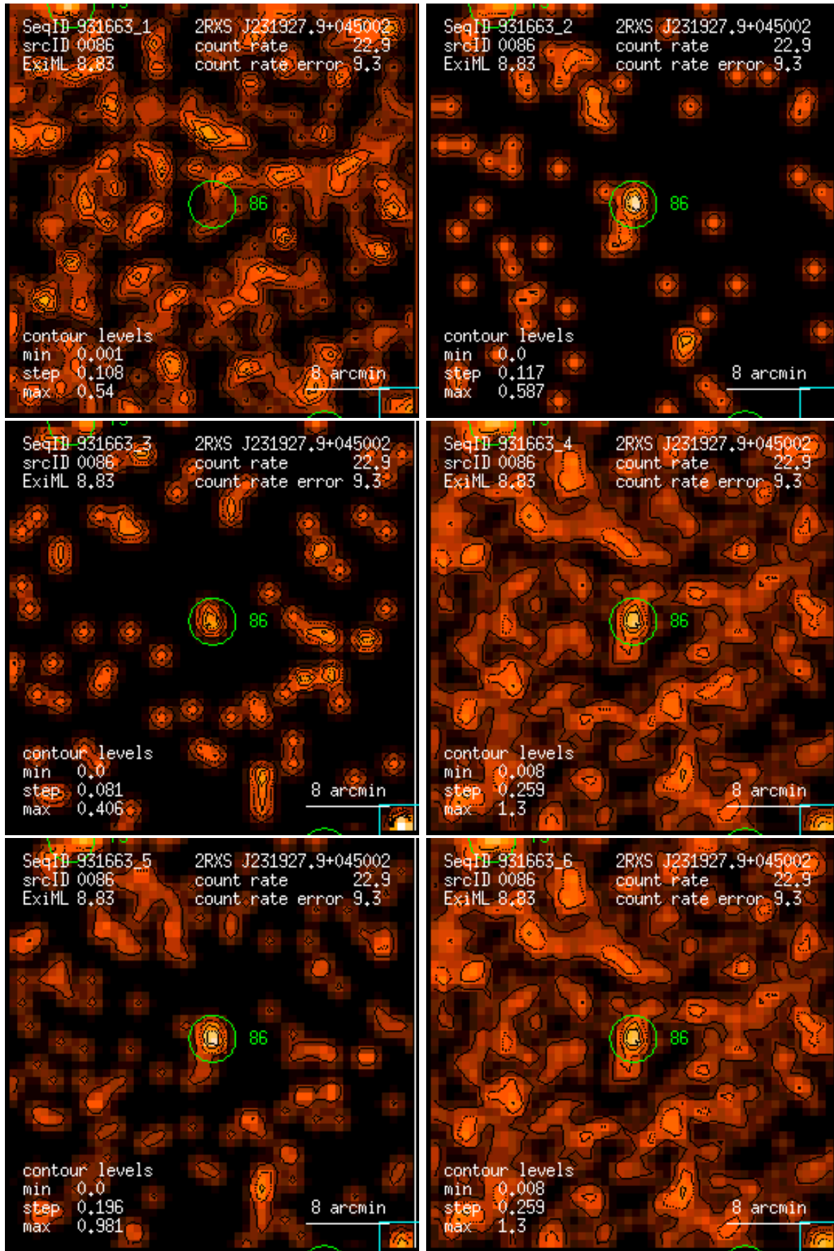
Figure 86: RASS 931663: detection 0086: band rate images, Gaussian filter: (1) PSPC channels 11 – 41, (2) 52 – 90, (3) 91 – 201, (4) 11 – 235, (5) 52 – 201, (6) 11 – 201. Broad band rates in counts/ks. Band rate contour levels in counts/ks/arcmin 2 .
