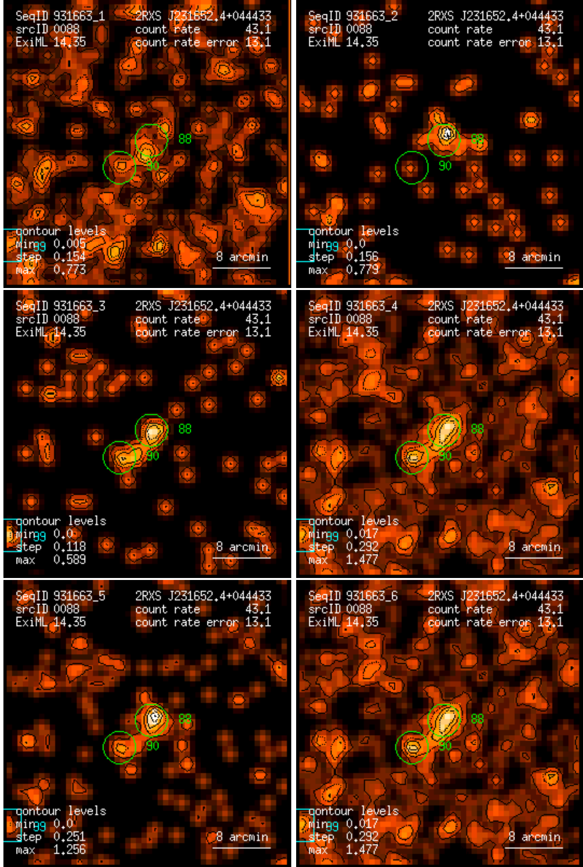
Figure 88: RASS 931663: detection 0088: band rate images, Gaussian filter: (1) PSPC channels 11 – 41, (2) 52 – 90, (3) 91 – 201, (4) 11 – 235, (5) 52 – 201, (6) 11 – 201. Broad band rates in counts/ks. Band rate contour levels in counts/ks/arcmin 2 .
