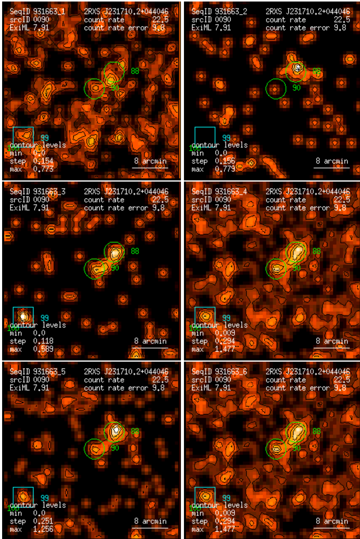
Figure 90: RASS 931663: detection 0090: band rate images, Gaussian filter: (1) PSPC channels 11 – 41, (2) 52 – 90, (3) 91 – 201, (4) 11 – 235, (5) 52 – 201, (6) 11 – 201. Broad band rates in counts/ks. Band rate contour levels in counts/ks/arcmin 2 .
