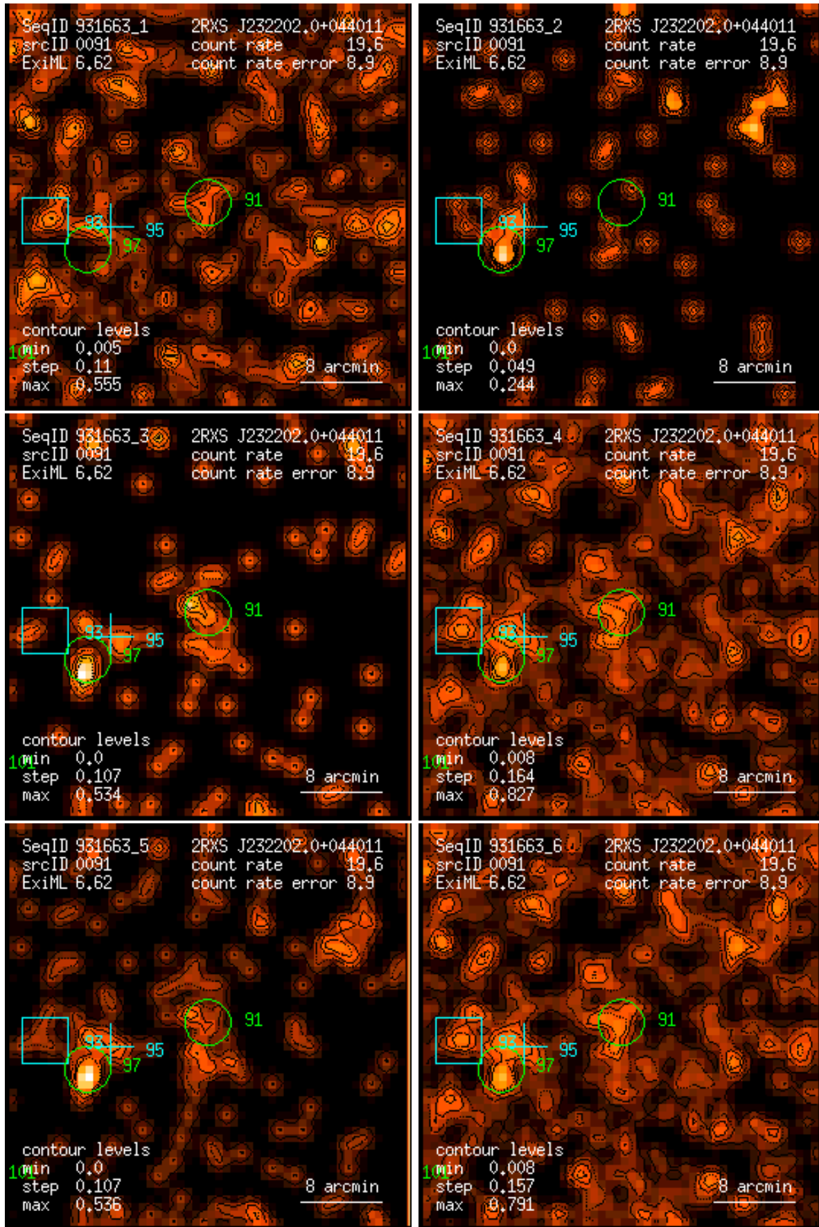
Figure 91: RASS 931663: detection 0091: band rate images, Gaussian filter: (1) PSPC channels 11 – 41, (2) 52 – 90, (3) 91 – 201, (4) 11 – 235, (5) 52 – 201, (6) 11 – 201. Broad band rates in counts/ks. Band rate contour levels in counts/ks/arcmin 2 .
