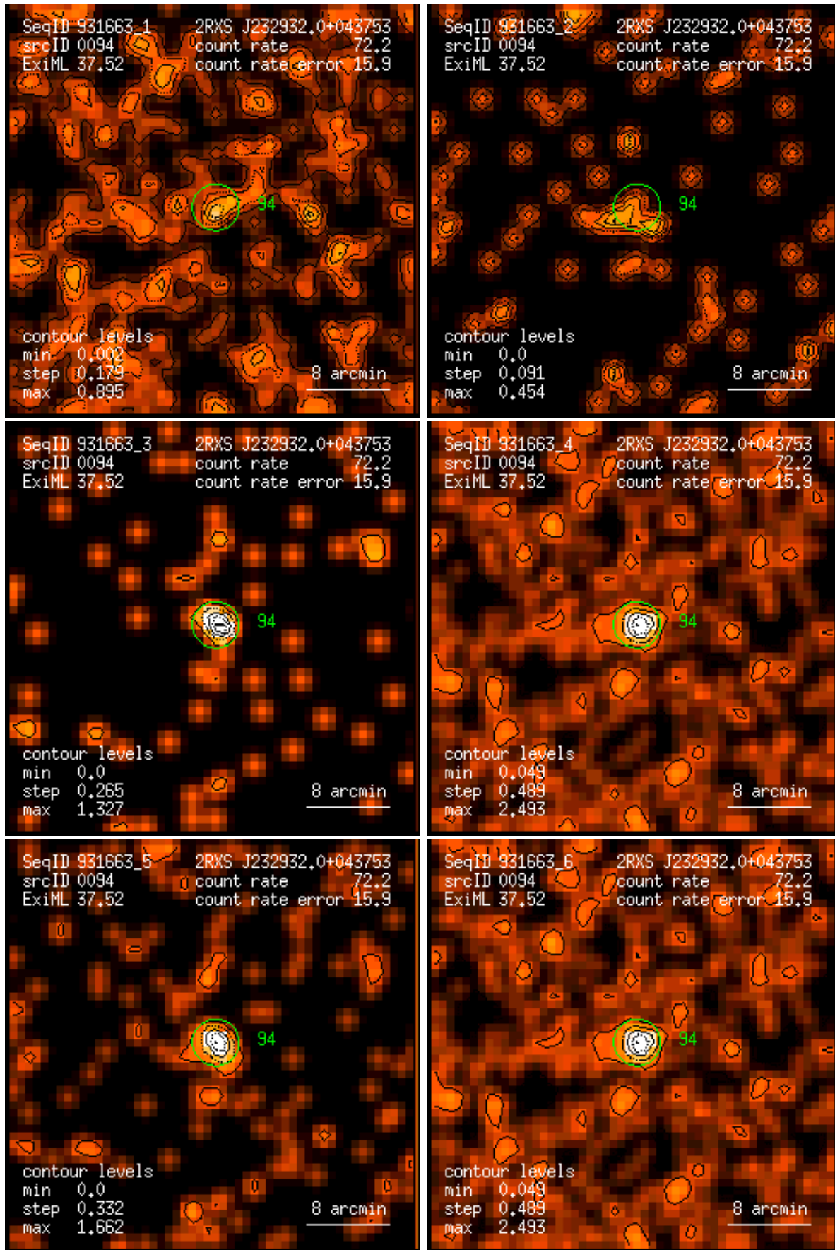
Figure 94: RASS 931663: detection 0094: band rate images, Gaussian filter: (1) PSPC channels 11 – 41, (2) 52 – 90, (3) 91 – 201, (4) 11 – 235, (5) 52 – 201, (6) 11 – 201. Broad band rates in counts/ks. Band rate contour levels in counts/ks/arcmin 2 .
