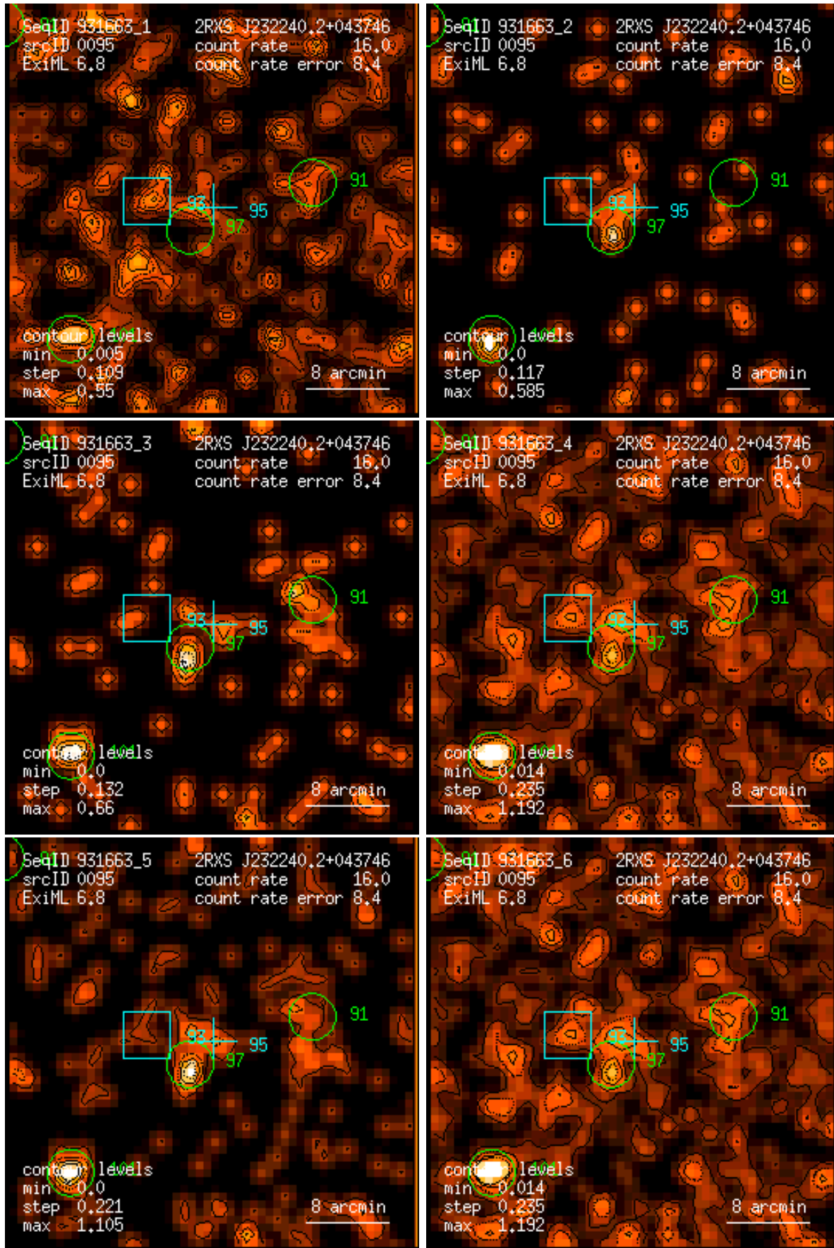
Figure 95: RASS 931663: detection 0095: band rate images, Gaussian filter: (1) PSPC channels 11 – 41, (2) 52 – 90, (3) 91 – 201, (4) 11 – 235, (5) 52 – 201, (6) 11 – 201. Broad band rates in counts/ks. Band rate contour levels in counts/ks/arcmin 2 .
