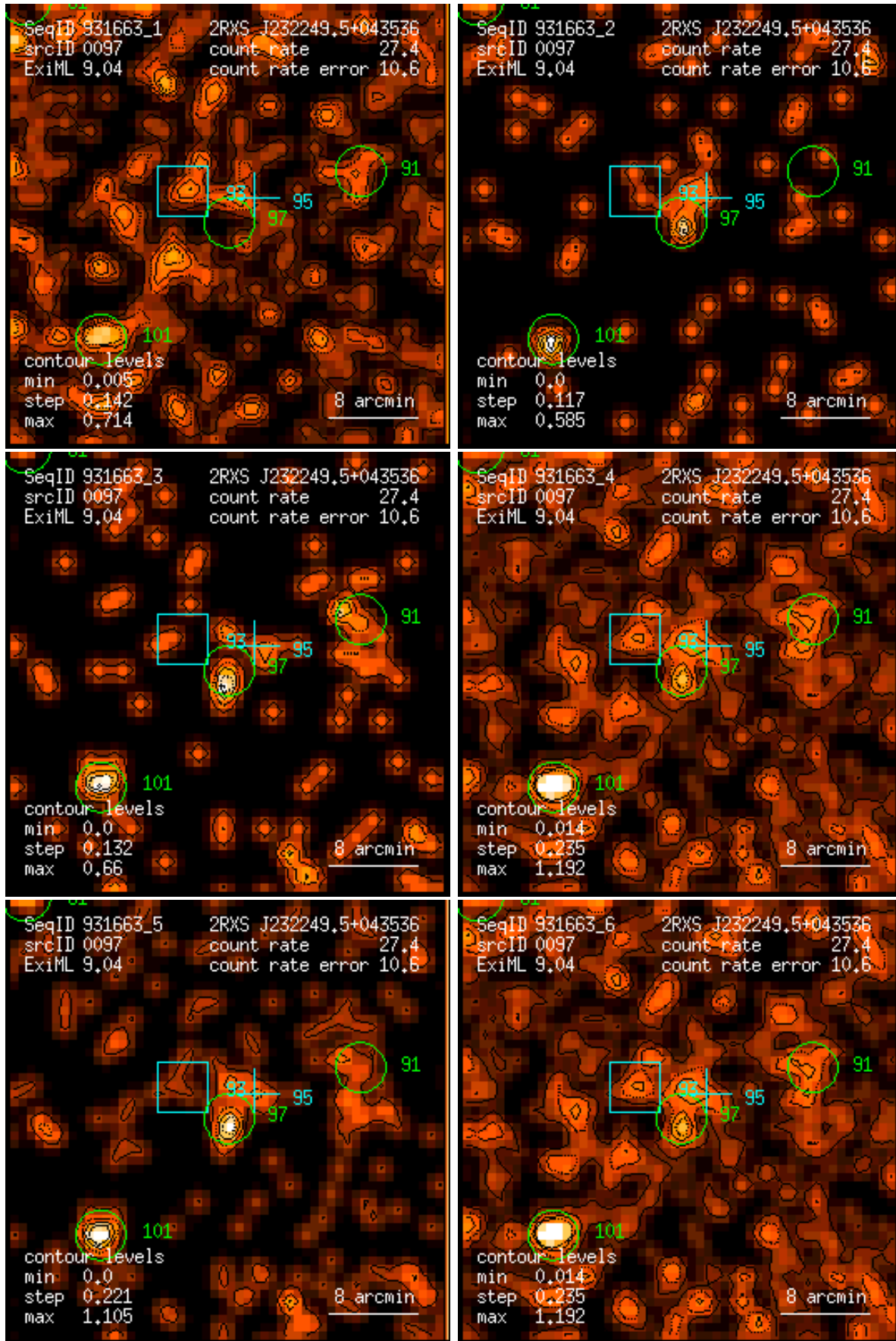
Figure 97: RASS 931663: detection 0097: band rate images, Gaussian filter: (1) PSPC channels 11 – 41, (2) 52 – 90, (3) 91 – 201, (4) 11 – 235, (5) 52 – 201, (6) 11 – 201. Broad band rates in counts/ks. Band rate contour levels in counts/ks/arcmin 2 .
