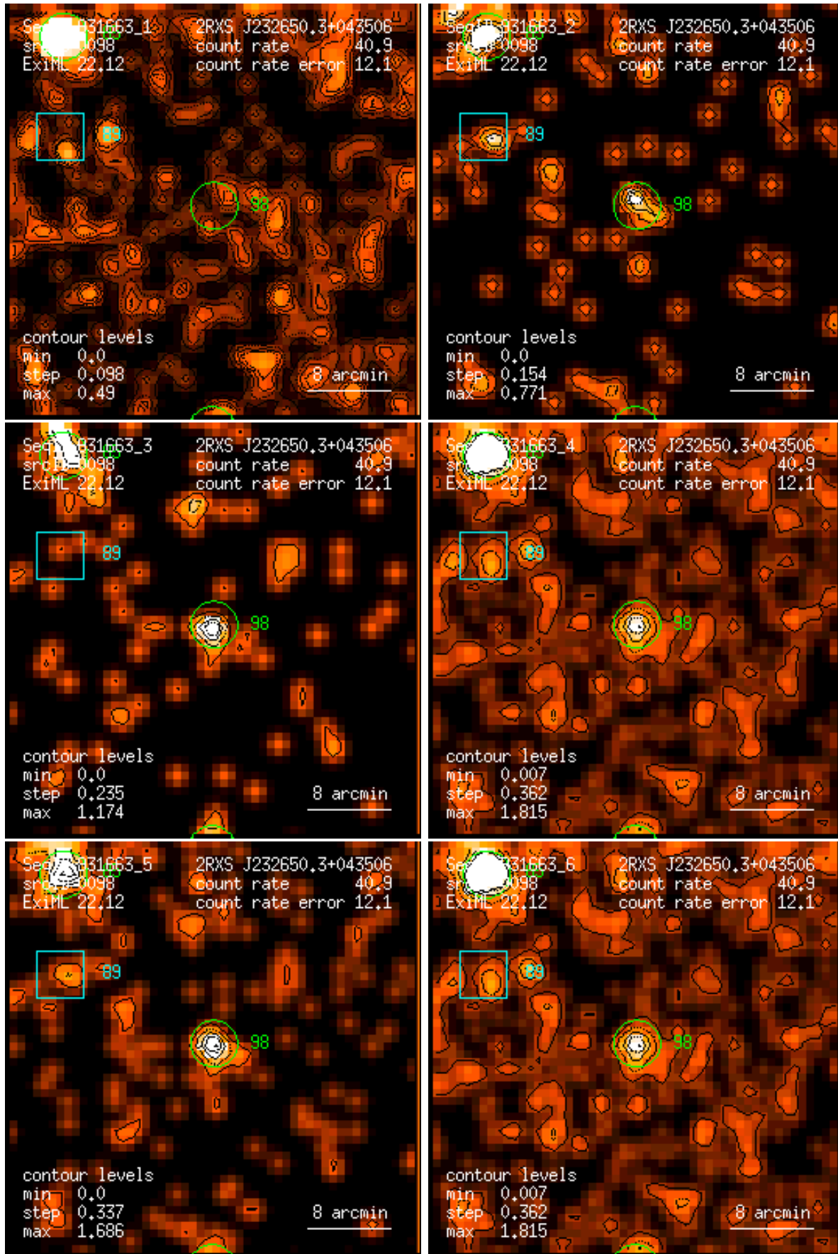
Figure 98: RASS 931663: detection 0098: band rate images, Gaussian filter: (1) PSPC channels 11 – 41, (2) 52 – 90, (3) 91 – 201, (4) 11 – 235, (5) 52 – 201, (6) 11 – 201. Broad band rates in counts/ks. Band rate contour levels in counts/ks/arcmin 2 .
