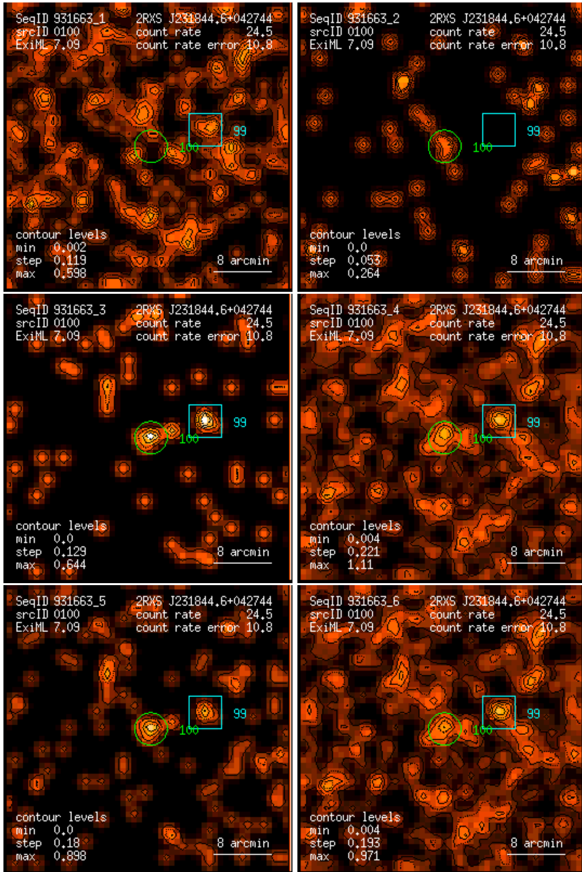
Figure 100: RASS 931663: detection 0100: band rate images, Gaussian filter: (1) PSPC channels 11 – 41, (2) 52 – 90, (3) 91 – 201, (4) 11 – 235, (5) 52 – 201, (6) 11 – 201. Broad band rates in counts/ks. Band rate contour levels in counts/ks/arcmin 2 .
