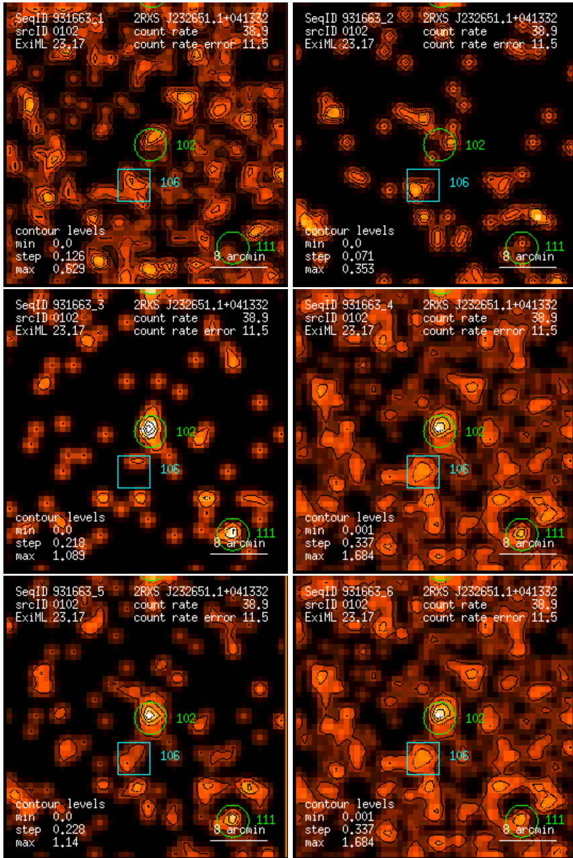
Figure 102: RASS 931663: detection 0102: band rate images, Gaussian filter: (1) PSPC channels 11 – 41, (2) 52 – 90, (3) 91 – 201, (4) 11 – 235, (5) 52 – 201, (6) 11 – 201. Broad band rates in counts/ks. Band rate contour levels in counts/ks/arcmin 2 .
