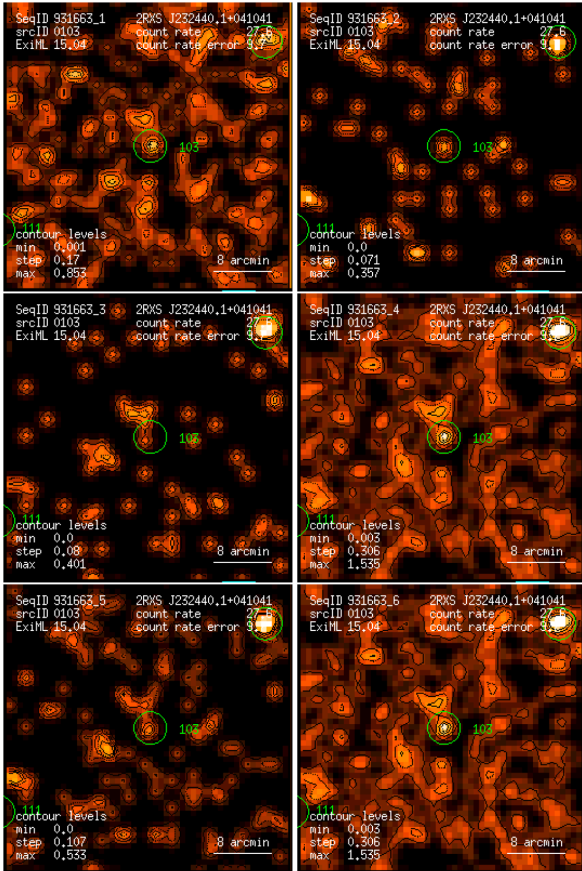
Figure 103: RASS 931663: detection 0103: band rate images, Gaussian filter: (1) PSPC channels 11 – 41, (2) 52 – 90, (3) 91 – 201, (4) 11 – 235, (5) 52 – 201, (6) 11 – 201. Broad band rates in counts/ks. Band rate contour levels in counts/ks/arcmin 2 .
