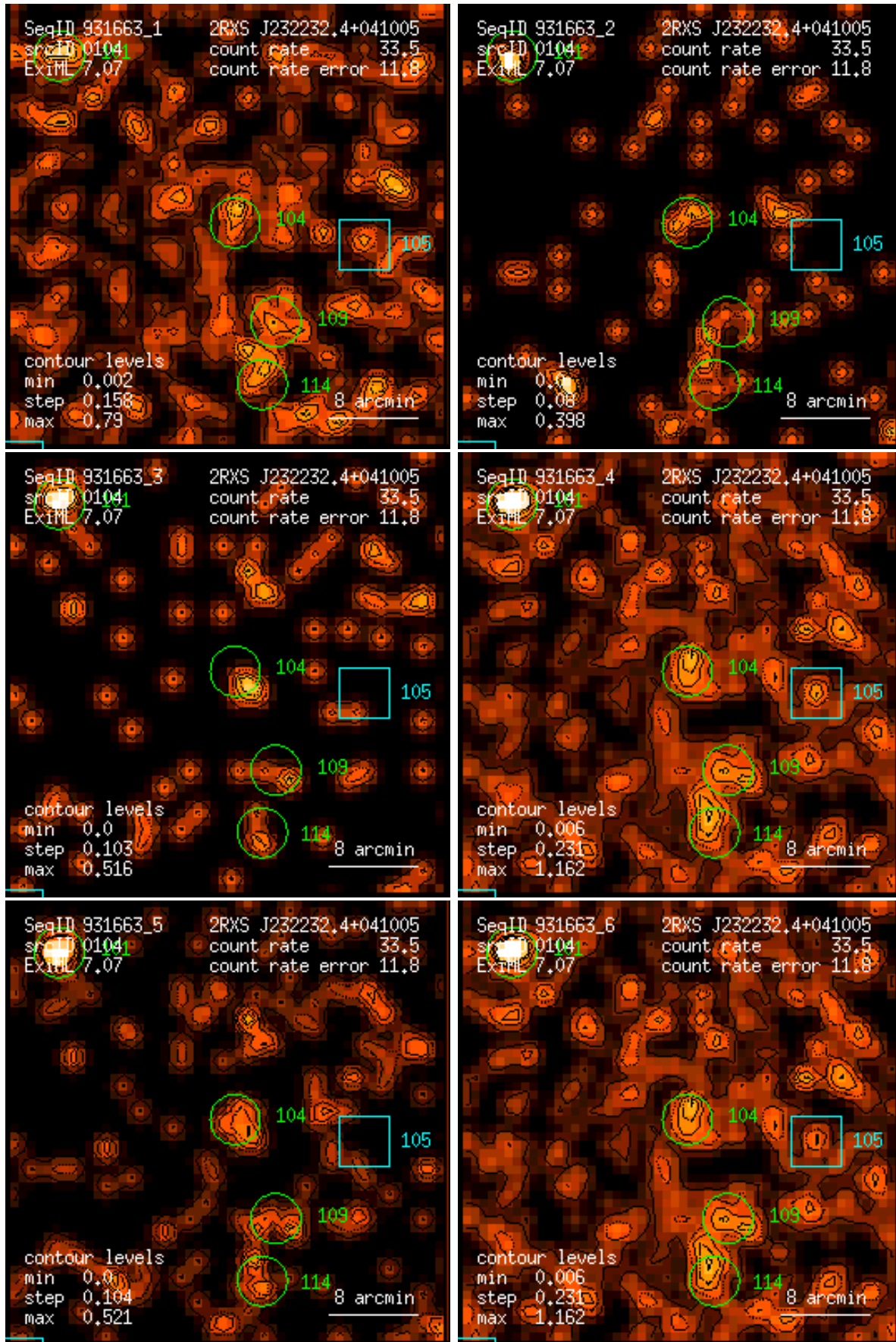
Figure 104: RASS 931663: detection 0104: band rate images, Gaussian filter: (1) PSPC channels 11 – 41, (2) 52 – 90, (3) 91 – 201, (4) 11 – 235, (5) 52 – 201, (6) 11 – 201. Broad band rates in counts/ks. Band rate contour levels in counts/ks/arcmin 2 .
