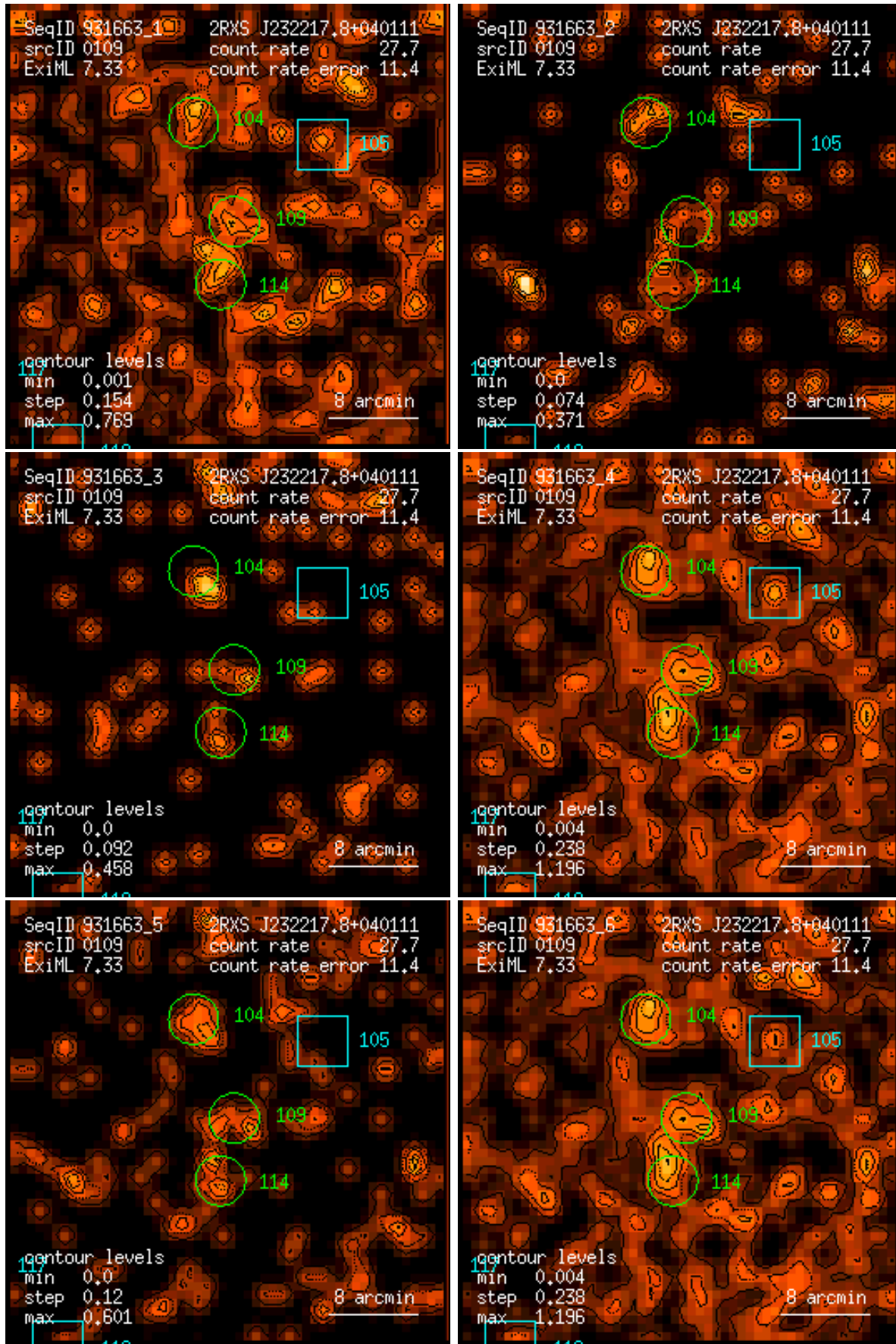
Figure 109: RASS 931663: detection 0109: band rate images, Gaussian filter: (1) PSPC channels 11 – 41, (2) 52 – 90, (3) 91 – 201, (4) 11 – 235, (5) 52 – 201, (6) 11 – 201. Broad band rates in counts/ks. Band rate contour levels in counts/ks/arcmin 2 .
