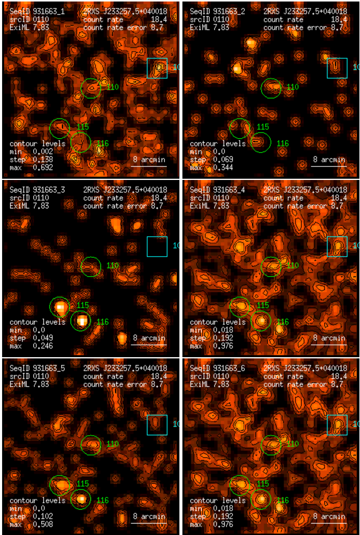
Figure 110: RASS 931663: detection 0110: band rate images, Gaussian filter: (1) PSPC channels 11 – 41, (2) 52 – 90, (3) 91 – 201, (4) 11 – 235, (5) 52 – 201, (6) 11 – 201. Broad band rates in counts/ks. Band rate contour levels in counts/ks/arcmin 2 .
