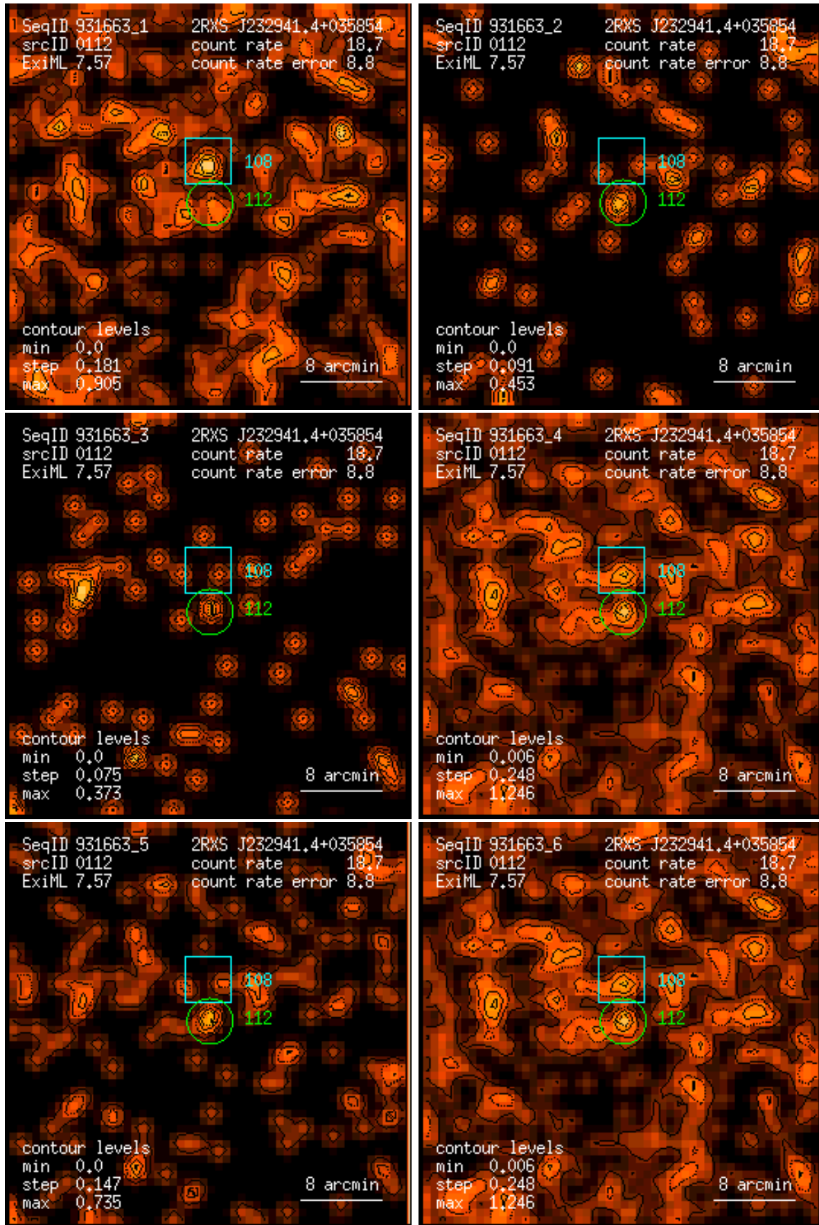
Figure 112: RASS 931663: detection 0112: band rate images, Gaussian filter: (1) PSPC channels 11 – 41, (2) 52 – 90, (3) 91 – 201, (4) 11 – 235, (5) 52 – 201, (6) 11 – 201. Broad band rates in counts/ks. Band rate contour levels in counts/ks/arcmin 2 .
