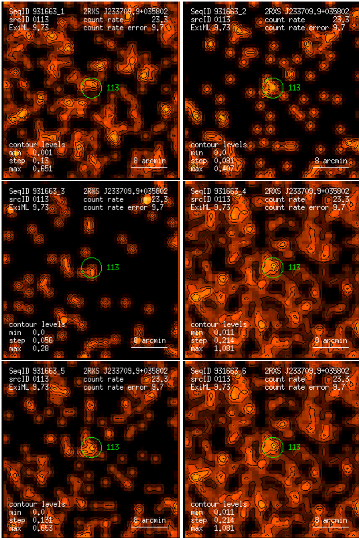
Figure 113: RASS 931663: detection 0113: band rate images, Gaussian filter: (1) PSPC channels 11 – 41, (2) 52 – 90, (3) 91 – 201, (4) 11 – 235, (5) 52 – 201, (6) 11 – 201. Broad band rates in counts/ks. Band rate contour levels in counts/ks/arcmin 2 .
