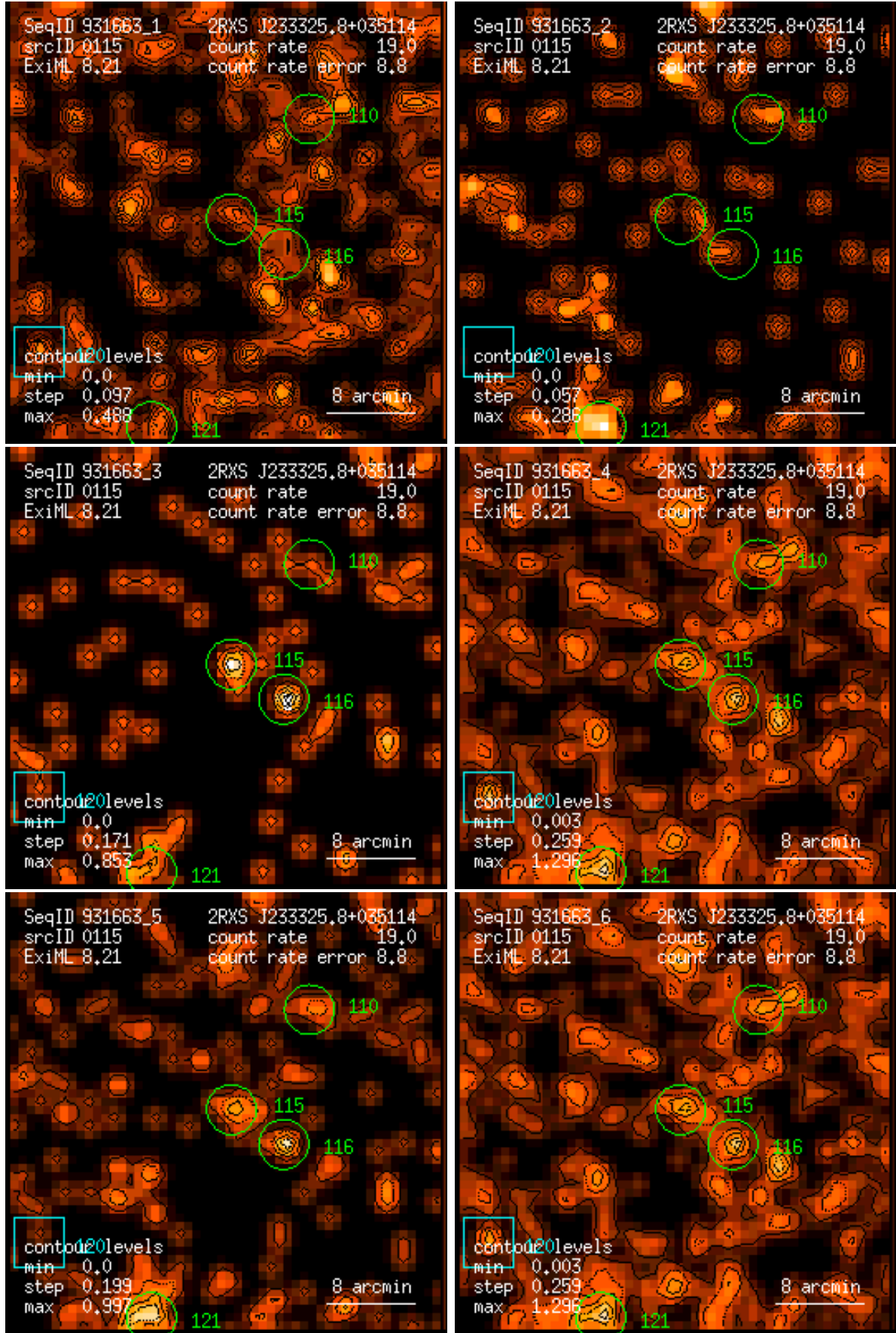
Figure 115: RASS 931663: detection 0115: band rate images, Gaussian filter: (1) PSPC channels 11 – 41, (2) 52 – 90, (3) 91 – 201, (4) 11 – 235, (5) 52 – 201, (6) 11 – 201. Broad band rates in counts/ks. Band rate contour levels in counts/ks/arcmin 2 .
