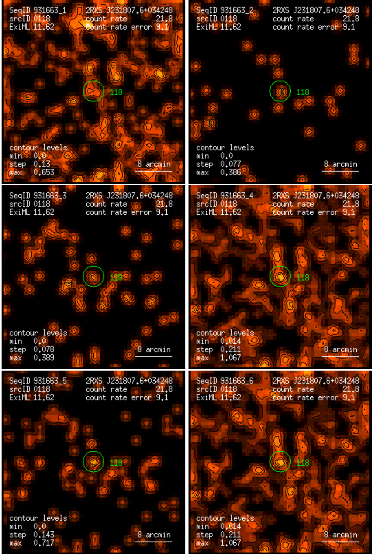
Figure 118: RASS 931663: detection 0118: band rate images, Gaussian filter: (1) PSPC channels 11 – 41, (2) 52 – 90, (3) 91 – 201, (4) 11 – 235, (5) 52 – 201, (6) 11 – 201. Broad band rates in counts/ks. Band rate contour levels in counts/ks/arcmin 2 .
