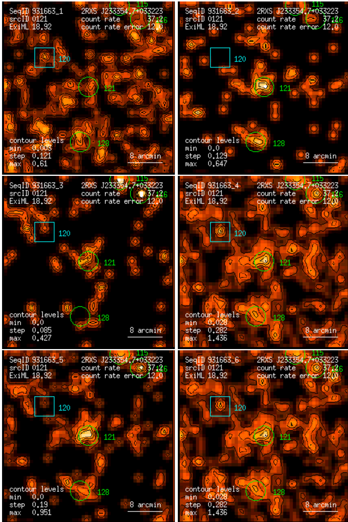
Figure 121: RASS 931663: detection 0121: band rate images, Gaussian filter: (1) PSPC channels 11 – 41, (2) 52 – 90, (3) 91 – 201, (4) 11 – 235, (5) 52 – 201, (6) 11 – 201. Broad band rates in counts/ks. Band rate contour levels in counts/ks/arcmin 2 .
