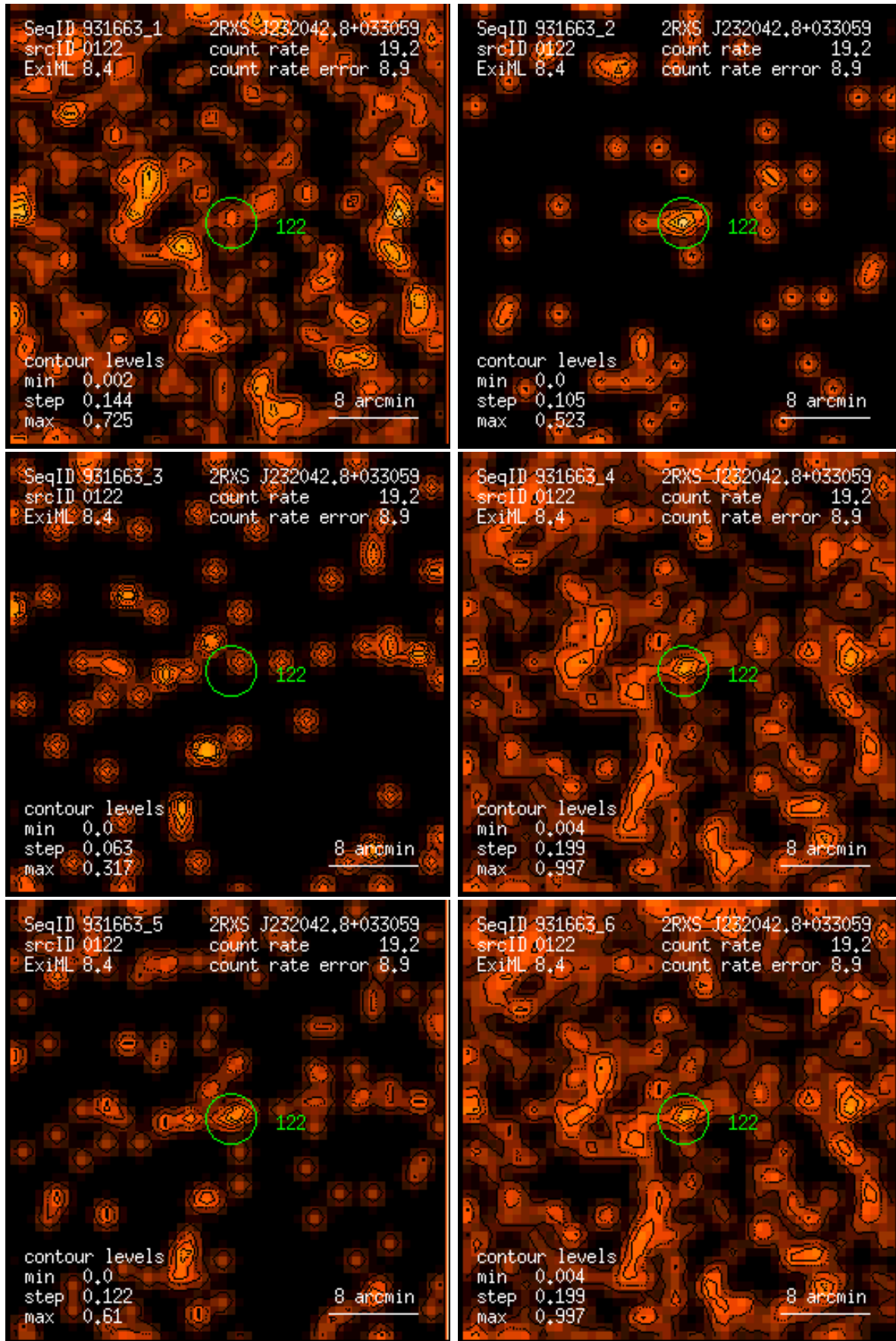
Figure 122: RASS 931663: detection 0122: band rate images, Gaussian filter: (1) PSPC channels 11 – 41, (2) 52 – 90, (3) 91 – 201, (4) 11 – 235, (5) 52 – 201, (6) 11 – 201. Broad band rates in counts/ks. Band rate contour levels in counts/ks/arcmin 2 .
