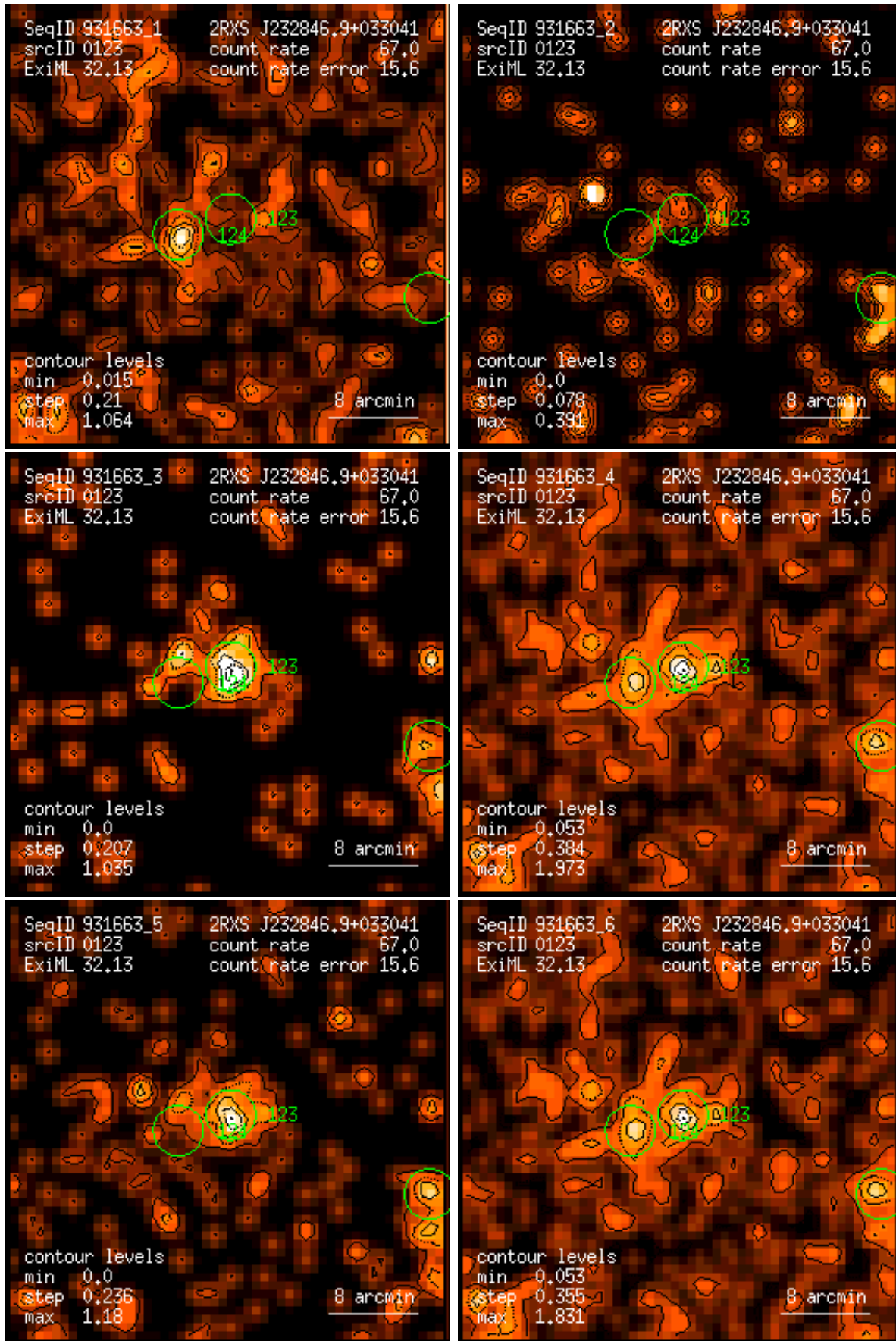
Figure 123: RASS 931663: detection 0123: band rate images, Gaussian filter: (1) PSPC channels 11 – 41, (2) 52 – 90, (3) 91 – 201, (4) 11 – 235, (5) 52 – 201, (6) 11 – 201. Broad band rates in counts/ks. Band rate contour levels in counts/ks/arcmin 2 .
