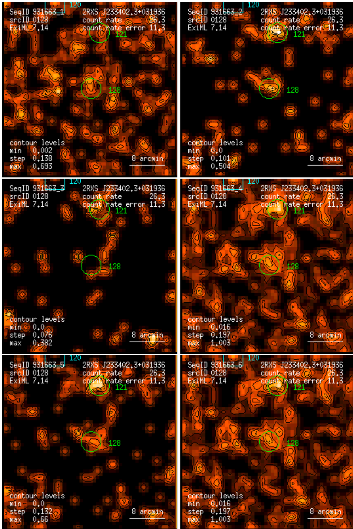
Figure 128: RASS 931663: detection 0128: band rate images, Gaussian filter: (1) PSPC channels 11 – 41, (2) 52 – 90, (3) 91 – 201, (4) 11 – 235, (5) 52 – 201, (6) 11 – 201. Broad band rates in counts/ks. Band rate contour levels in counts/ks/arcmin 2 .
