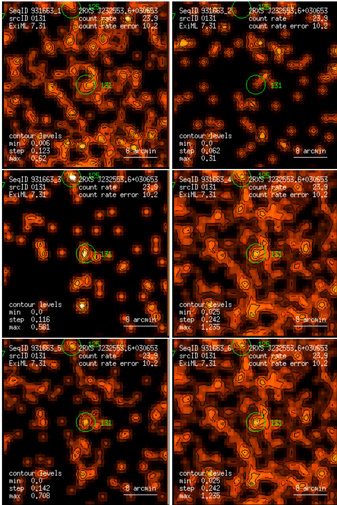
Figure 131: RASS 931663: detection 0131: band rate images, Gaussian filter: (1) PSPC channels 11 – 41, (2) 52 – 90, (3) 91 – 201, (4) 11 – 235, (5) 52 – 201, (6) 11 – 201. Broad band rates in counts/ks. Band rate contour levels in counts/ks/arcmin 2 .
