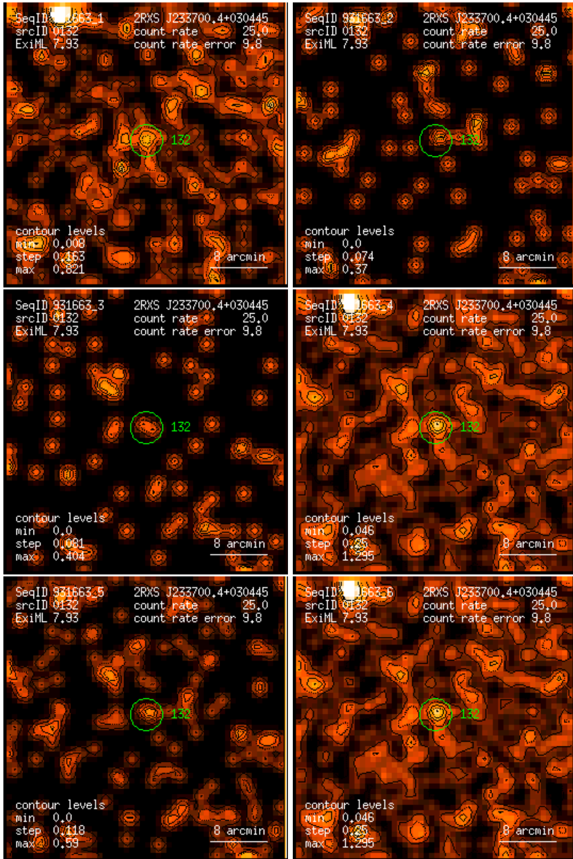
Figure 132: RASS 931663: detection 0132: band rate images, Gaussian filter: (1) PSPC channels 11 – 41, (2) 52 – 90, (3) 91 – 201, (4) 11 – 235, (5) 52 – 201, (6) 11 – 201. Broad band rates in counts/ks. Band rate contour levels in counts/ks/arcmin 2 .
